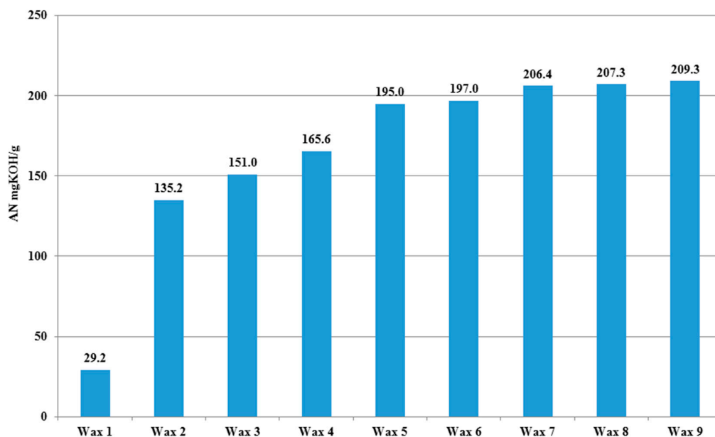
Figure 1. Acid number (AN) of O-PEW obtained in the melt phase oxidation process.
