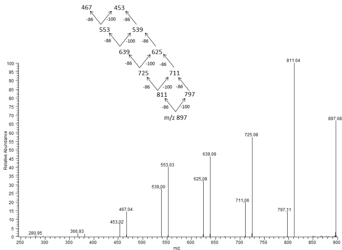
Figure 6. ESI-MS/MS spectrum obtained for the selected sodium adduct of oligomers [\text{HB}_9 \text{HV} + \text{Na}]^+ at m/z 897.
