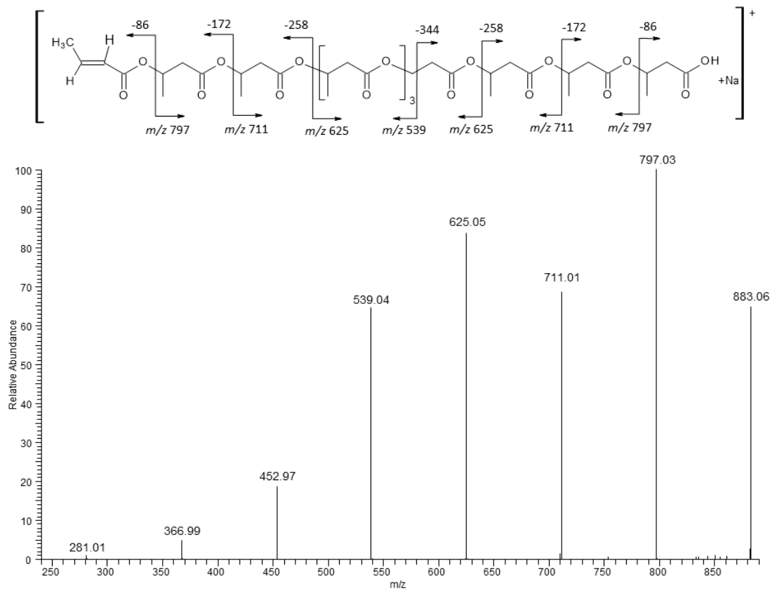
Figure 5. ESI-MS/MS spectrum obtained for the selected sodium adduct ion of oligomers in [\text{HB}_{10} + \text{Na}]^+ m/z 883.
