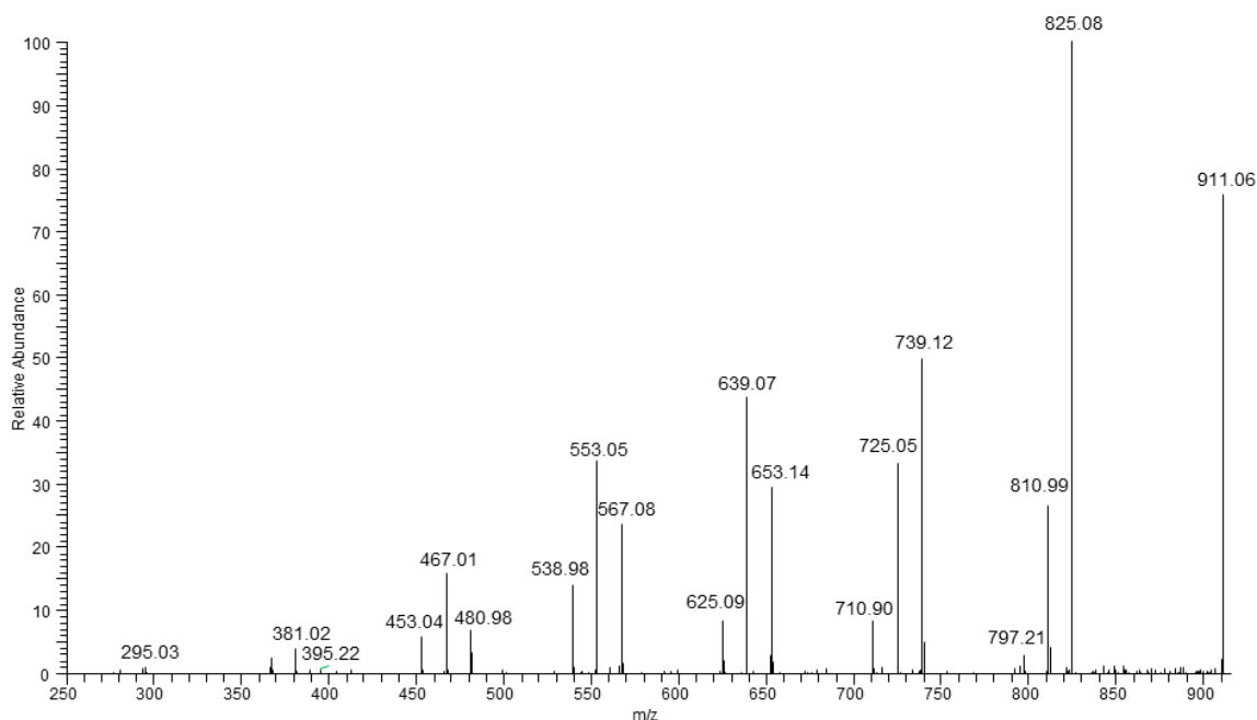
Figure 7. ESI-MS/MS spectrum obtained for the selected sodium adduct of oligomers at m/z 911.
