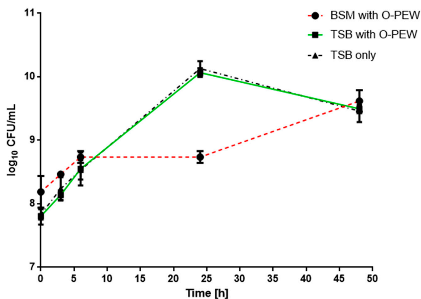
Figure 2. Small-scale shake-flasks experiments of R. eutropha H16 with 5 g/L of O-PEW in TSB (green line, black squares) or BSM (red line, black circles) and TSB only (black line, black triangles). Viable count ( \log_{10} CFU/mL) data points at time 0, 3, 6, 24, and 48 h are the arithmetic means of triplicates, while error bars represent the standard error (SE) of the mean.
