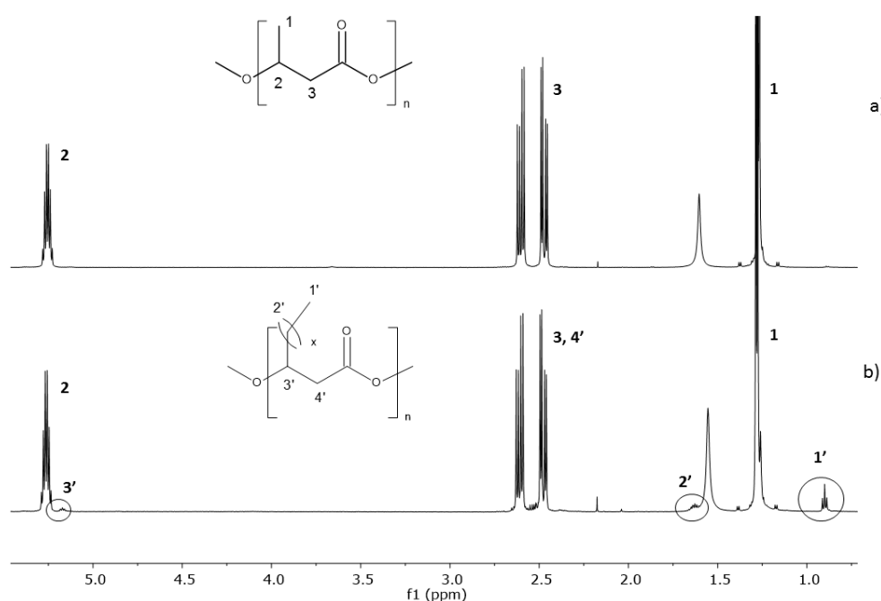
Figure 3. ^1\text{H-NMR} spectra of the polyesters obtained via fermentation of R. eutropha H16 with the use of (a) TSB; and (b) TSB/O-PEW as an additional carbon sources.
