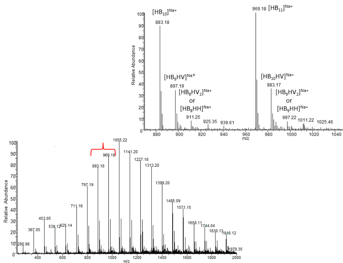
Figure 4. The ESI-MS spectrum (positive-ion mode) of the PHA oligomers, obtained via partial thermal degradation of the biopolyester obtained using TSB/O-PEW as a carbon source, together with an extended spectral range of m/z 870–1050.
