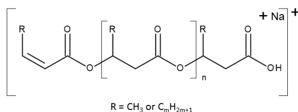
Scheme 1. General formula of ions observed in ESI-MS spectra.
