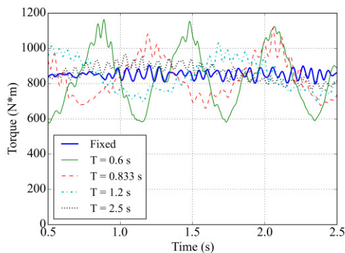
(b) Torque
