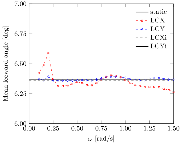
Fig. 9. Mean leeward angles obtained from wind-and-wave dynamic simulations.
