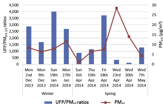
Fig. 4. Ratios between median UFP and PM 0.5-2.5 concentrations and average PM 2.5 concentration measured by TEOM-FDMS on each day. The ratios in the spring campaign were calculated from the static measurements. The same instruments were used to calculate the ratios in the winter campaign for the purpose of comparison between the ratios in the two campaigns.
