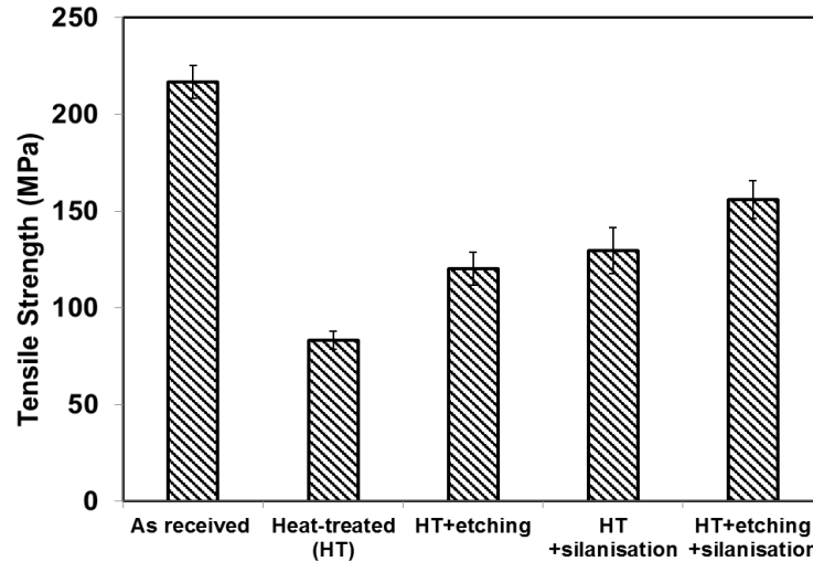
Figure 5 Tensile strength of CSM-epoxy composites with glass fibres received different treatments
