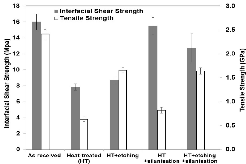
Figure 3 Interfacial shear strength of GF-mPP and tensile strength of GF after different fibre treatments including heat-treated: 500°C for 25 minutes, etching: immersion in 1 v% HF solution for 2.5 minutes, and silanisation: immersion in 1 v% APS for 15 minutes
