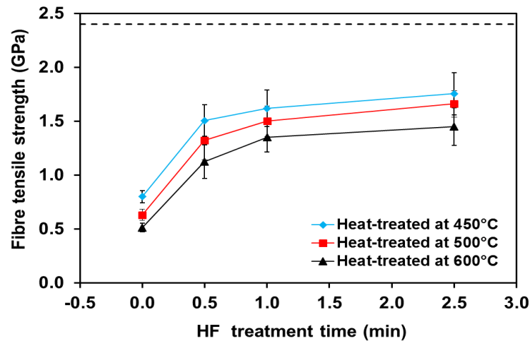
Figure 1 Tensile strength of heat-treated glass fibres as a function of the treatment time of 1 v% of HF aqueous solution
