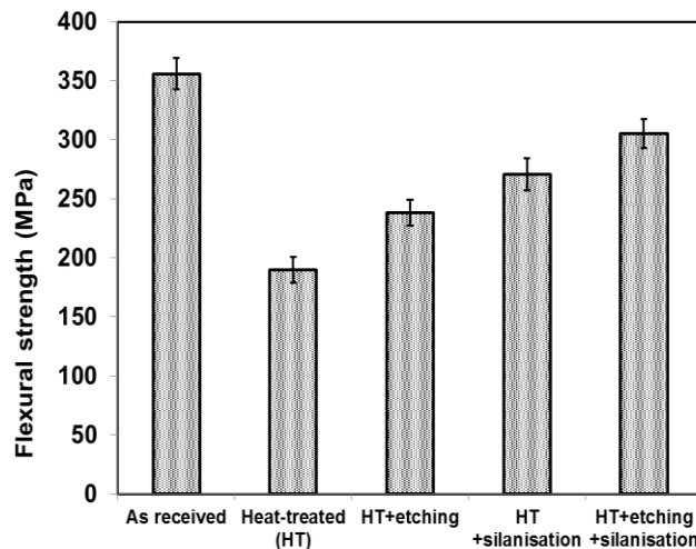
Figure 7 Flexural strength of CSM-epoxy composites with glass fibres received different treatments
