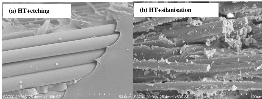
Figure 6 SEM photo of fractured area obtained from tested samples consisting of the CSM conditioned with (a) heat treatment at 500°C followed by HF etching and (b) the same heat treatment followed by APS silanisation
