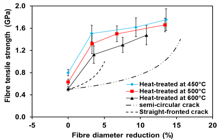
Figure 2 Tensile strength of heat-treated glass fibres as a function of fibre diameter reduction
