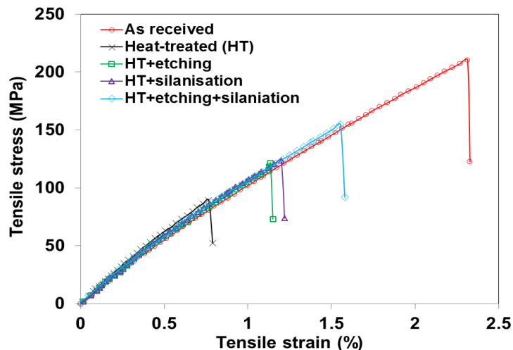
Fig 4 Typical tensile stress-strain curve obtained from CSM-epoxy composites with glass fibres received different treatments
