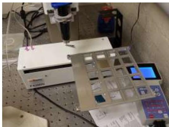
Figure 4. Holder plate with space for 20 array mounts. Positional accuracy was specified to be better than 200 \mu m in x & y.
