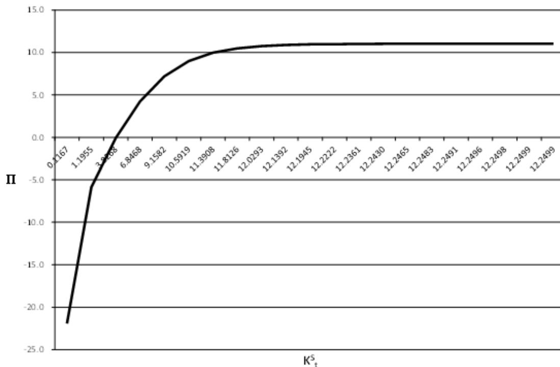
Figure 4.13: The deviation value of banks to risky investment when \theta = 3.0
