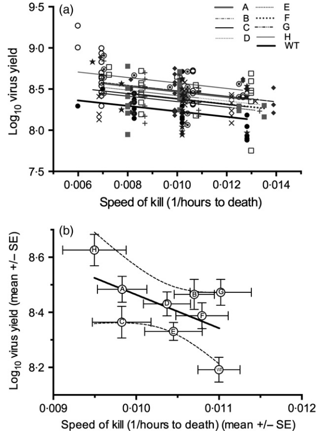
Fig. 3. Yield speed of kill trade-offs for individual SpexNPV genotypes and the wild-type virus at the (a) intra-genotype level (genotype A \odot , B \square , C \square , D + , E \times , F \blacksquare , G \blacklozenge , H \circ and WT \bullet ) and (b) inter-genotype level. In (b), mean speed of kill was estimated only using larvae for which virus yield data were also available.
