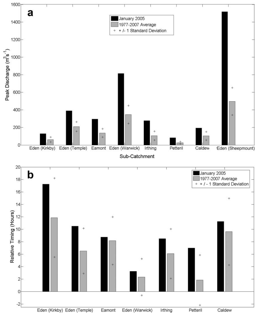
Figure 4. Comparison of the January 2005 flood with the long-term average in terms of peak magnitudes from each subwatershed. Comparison of the January 2005 flood with the long-term average in terms of the peak flow relative timing from each subwatershed with respect to Carlisle. A value of 0 means that both the tributary and the downstream main river peak at the same time.
