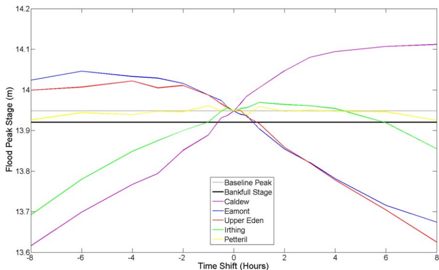
Figure 6. Sensitivity of peak stage at Carlisle (Sheepmount) to timing shifts of the contributing subwatershed's hydrograph—light gray line = original peak flow, dark gray line = bank full.
