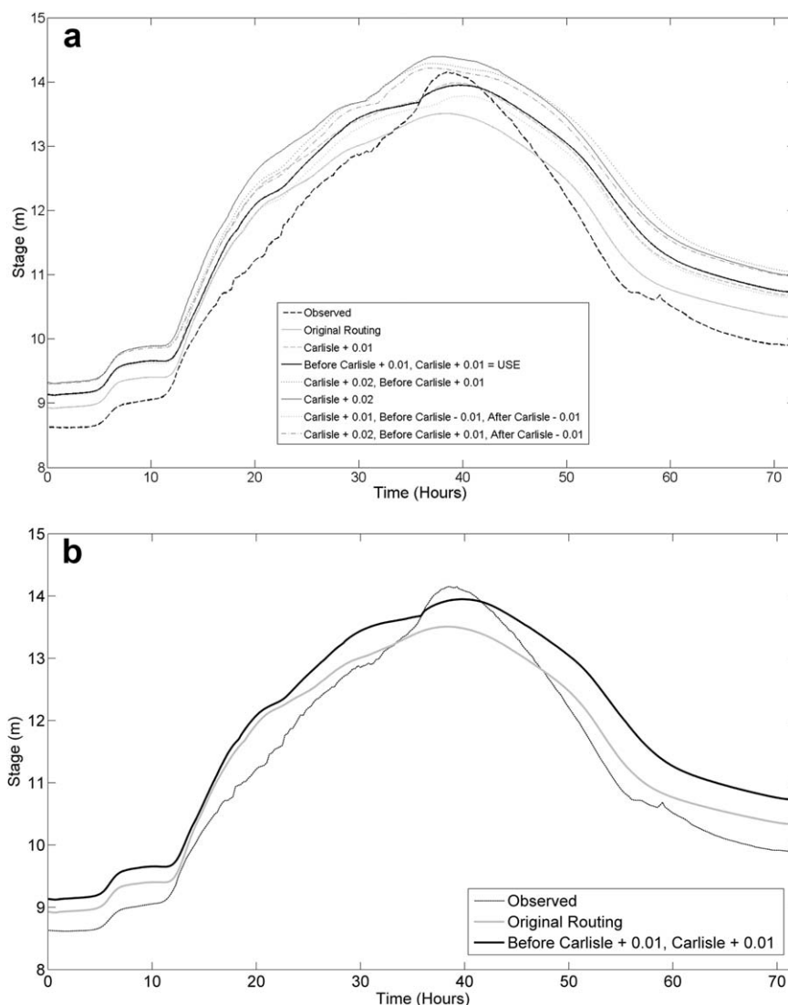
Figure 3. Sensitivity analysis of Sheepmount hydrograph to Manning’s n. Simulations represent changing Manning’s n in different reaches of Eden, e.g., U/S tribis (before –0.01, Carlisle +0.01 = Manning’s n decreased by 0.01 before Carlisle and increased by 0.01 in Carlisle itself. Calibration of Eden iSIS model using downstream gauging station of Sheepmount in Carlisle to optimize for flood peak. (Performance statistics – Nash Sutcliffe Coefficient = 0.85, RMSE = 0.67 m, % error peak stage = –1.45%, % error in volume = 5.2%)
