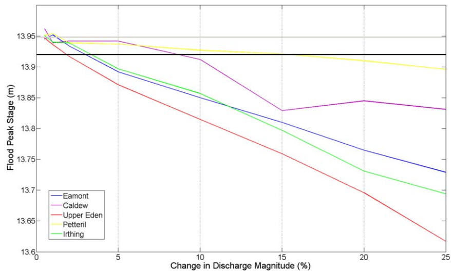
Figure 5. Sensitivity of peak stage at Carlisle (Sheepmount) to percentage decreases in subwatershed hydrograph contributions.
