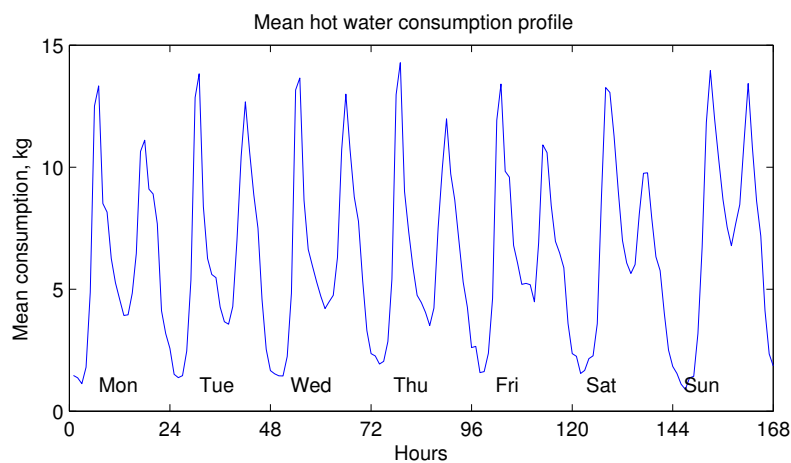
Figure 8. Weekly mean hot water consumption pattern [32].
