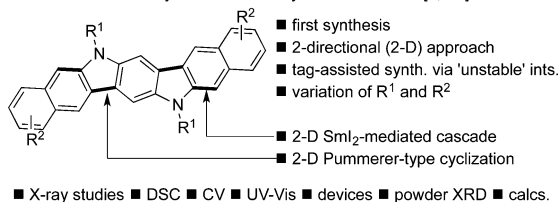
Figure 1. (A) Indolo[3,2- b ]carbazole motif in organic semiconductors. (B) Unknown dibenzoindolo[3,2- b ]carbazole (DBIC) motif. (C) This study: 2-D, tag-assisted synthesis and study of DBICs.
