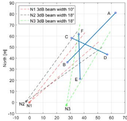
Fig. 1. Experimental setup and birds flight paths
