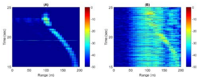
Fig. 9. RTI signatures of DJI Phantom quadcopter drone moving from A to B (A) Monostatic HH (B) Monostatic HV (C) Bistatic HH
