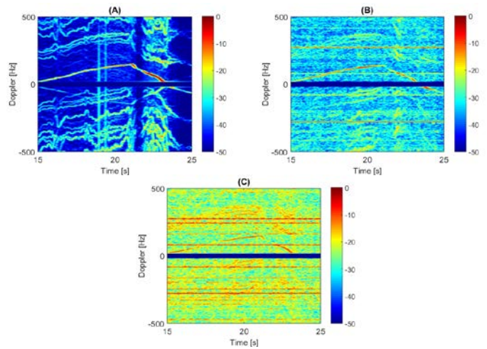
Fig. 10. Micro-Doppler signatures of DJI Phantom quadcopter drone moving from A to B (A) Monostatic HH (B) Monostatic HV (C) Bistatic HH
