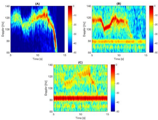
Fig. 8. Micro-Doppler signature of Barn Owl moving from A to B (A) Monostatic HH (B) Bistatic HH (C) Monostatic HV
