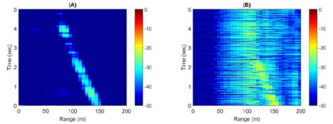
Fig. 6. RTI of Eurasian Eagle Owl moving from A to B (A) Monostatic HH (B) Bistatic HH
