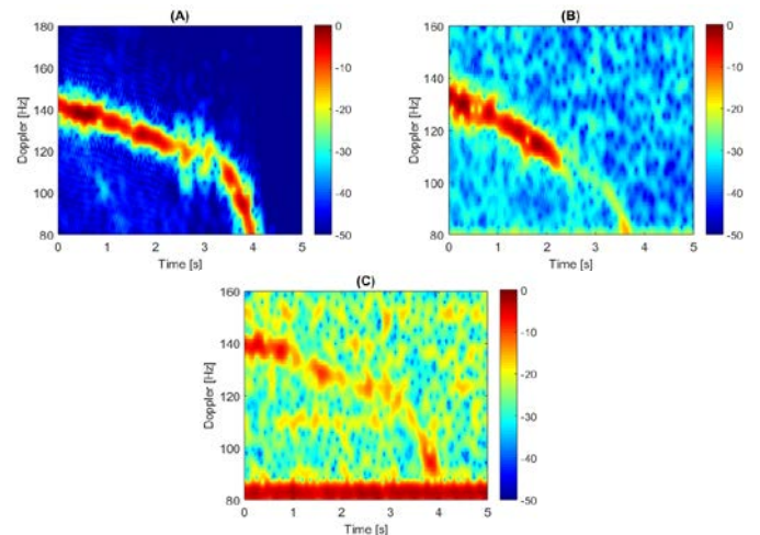
Fig. 7. Micro-Doppler signature of Eurasian Eagle Owl moving from A to B (A) Monostatic HH (B) Bistatic HH (C) Monostatic HV
