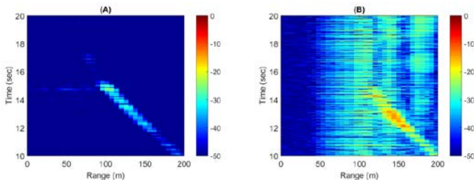
Fig. 4. RTI of Hooded Vulture moving from A to B (A) Monostatic HH (B) Bistatic HH
