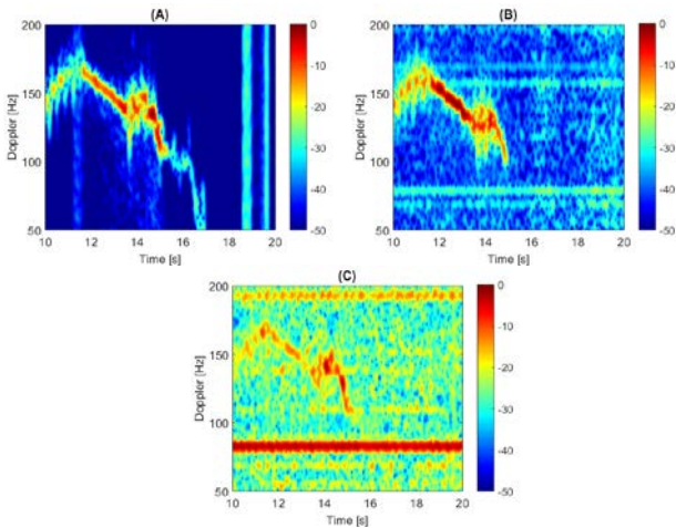
Fig. 5. RTI of Hooded Vulture moving from A to B (A) Monostatic HH (B) Bistatic HH (C) Monostatic HV
