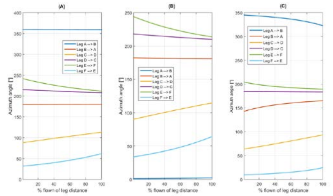
Fig. 2. Actual aspect angle of birds in flight dependent on flight path with respect to the radar nodes (a) Node 1 (b) Node 2 (c) Node 3
