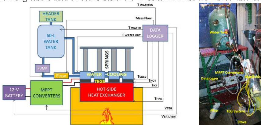
Fig. 1. Diagram (left) and picture (right) of the experimental system.
