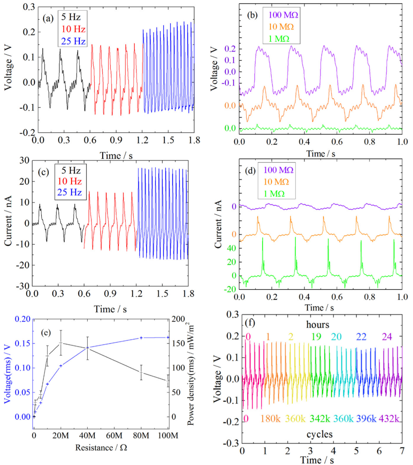
Figure 4. Electrical output of the ZnO-PC nanogenerator. (a) Voltage output at different frequencies of impact vibrations measured across a 20\text{ M}\Omega resistor and (b) the voltage across different loads at 5\text{ Hz} . (c) Current output at different frequencies measured through a 20\text{ M}\Omega resistor and (d) the current through different resistors at 5\text{ Hz} . (e) Root-mean-square voltage measured over ten different resistors and the corresponding power density of a single device and (f) the voltage output measured across a 10\text{ M}\Omega resistor at 5\text{ Hz} after 1, 2, 19, 22 and 24 h. The amplitude of the impacting vibrations is frequency-dependent and for 5\text{ Hz} , 10\text{ Hz} and 25\text{ Hz} are 0.68\text{ mm} , 0.65\text{ mm} , 0.78\text{ mm} respectively.
