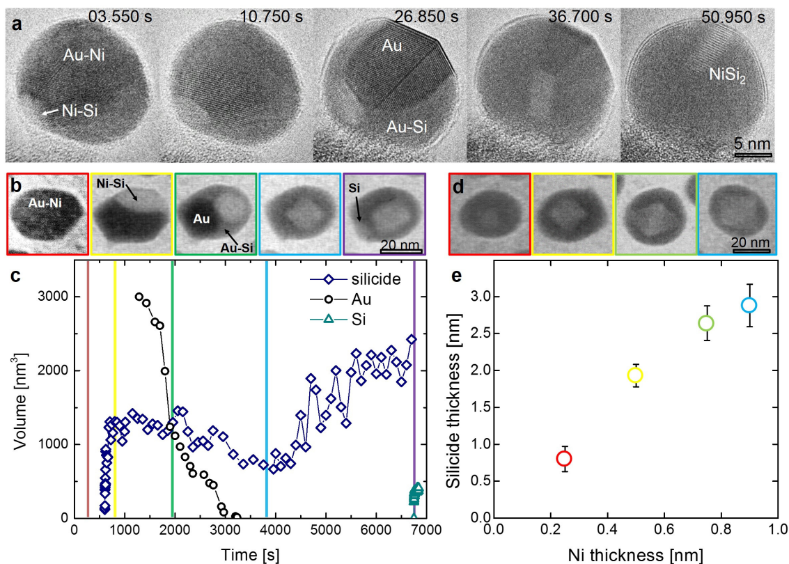
Figure 3: Ni-silicide nucleation in AuNi nanocrystals deposited on Si nitride membranes. a The sequence of phases observed in situ in ETEM during exposure of a 7 nm radius polycrystalline Au aerosol particle covered with 0.1 nm of Ni to 3.5 \times 10^{-5} Torr of \text{Si}_2\text{H}_6 at 400^\circ\text{C} . The characteristic shape of \text{NiSi}_2 is first visible in the fourth image. b Sequence observed in UHVTEM during exposure of a 15 nm radius polycrystalline Au-Ni crystallite to 3.5 \times 10^{-8} Torr \text{Si}_2\text{H}_6 at 490^\circ\text{C} . 2.5 nm Au followed by 0.5 nm Ni were evaporated onto a silicon nitride membrane (see Methods) and agglomerated by annealing in vacuum. c Volume versus time of each phase calculated from the projected area and assuming a height equal to the average diameter. Note that the initial silicide volume is overestimated because its shape is far from the assumed ellipsoid; values obtained after disappearance of solid Au are more likely to be accurate. Colored vertical lines identify the time corresponding to images in c . d Sequence of images of average size silicides formed after the process in b , but starting with different amounts of Ni. e Colour-coded data of silicide thickness vs. thickness of deposited Ni corresponding to the images in d . Silicide thickness is measured by adding the estimated volume of all the silicide nanocrystals recorded in a frame and dividing by its area. Error bar represents the standard deviation calculated by measuring the silicide thickness in 5 different frames.
