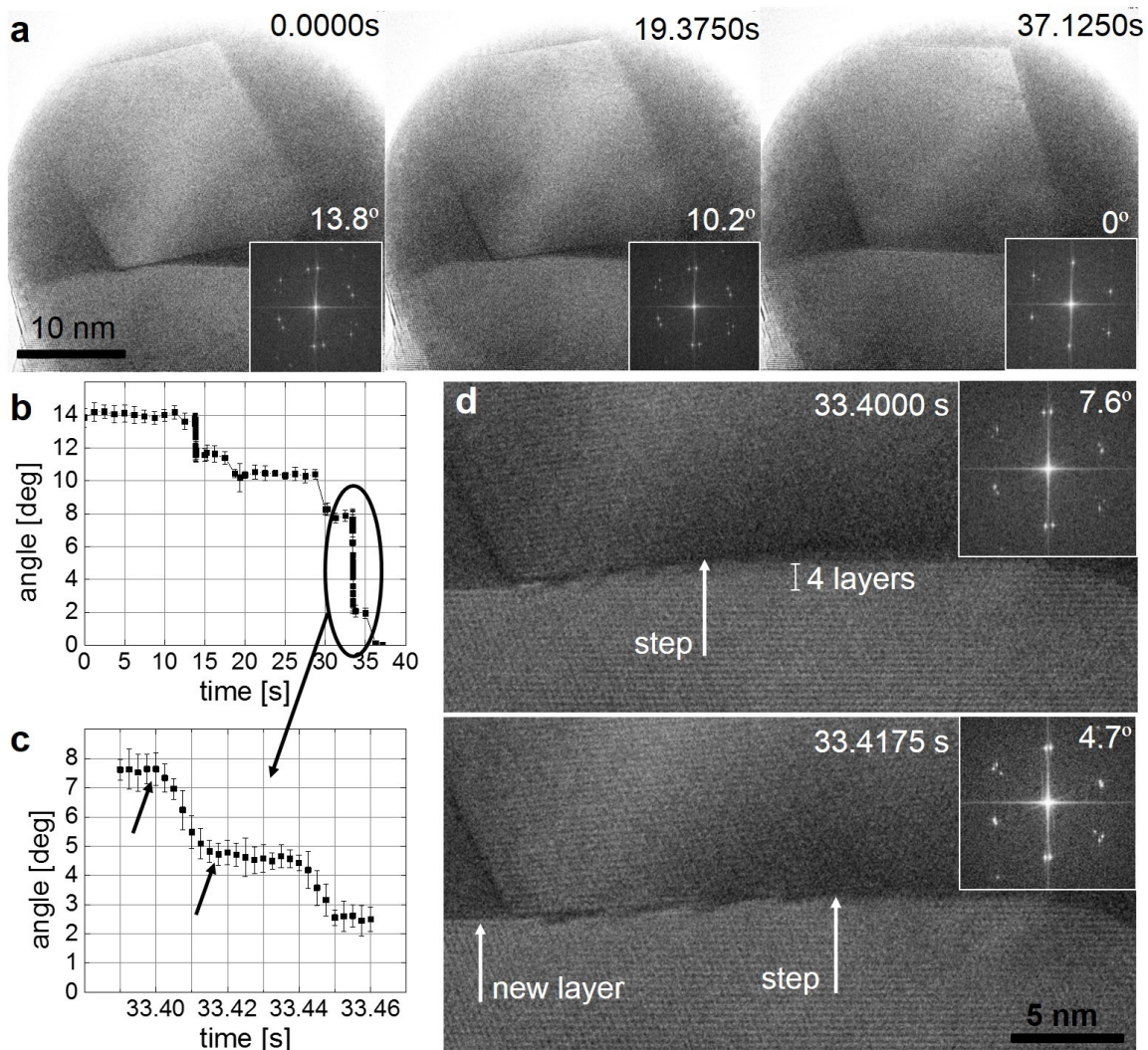
Figure 2: The docking of a silicide particle with its nanowire. a Sequence of atomically resolved, 400 fps TEM images recorded at 400°C. The insets show the FFT of each respective image with the angle between the two crystals indicated. b The rotation angle measured from the FFT of the image series in a and Movie 2. c Detail of b showing one larger rotation occurring in two distinct increments; arrows indicate the data corresponding to the images in d . d Detail of the sequence in a showing rearrangement of the Si surface during silicide rotation. The insets show the respective FFTs.
