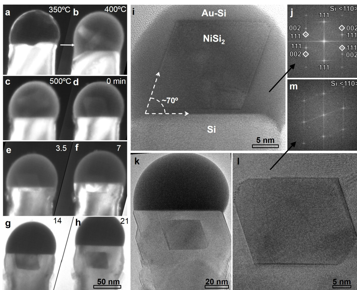
Figure 1: TEM images showing nickel silicide formation and incorporation in Si nanowires. a-d Sequence of dark field (DF) images recorded after Ni deposition and oxidation, while raising the temperature to 500°C in 5 \times 10^{-5} Torr Si 2 H 6 . A NiSi 2 nanocrystal forms inside the AuSi droplet and makes epitaxial contact with Si. The arrow in b shows the initial Au/Si interface. e-h Nanowire growth that embeds the nanocrystal as the temperature reaches 500°C. The growth rate is steady, apart from in the first few minutes where it is slowed, perhaps by impurities formed at the catalyst surface during oxidation. Bright field conditions are used in g and h to highlight the structure. The time is given in seconds. i, j High-resolution image and Fast Fourier transform (FFT) of a different nanowire showing a nanocrystal in a twinned epitaxial relation with Si. k, l, m Image, detail and FFT showing endotaxy in a different nanowire in which the process of silicide incorporation is completed. The dark and bright lines around the nanocrystal in panel l are due to diffraction at the crystal interfaces.
