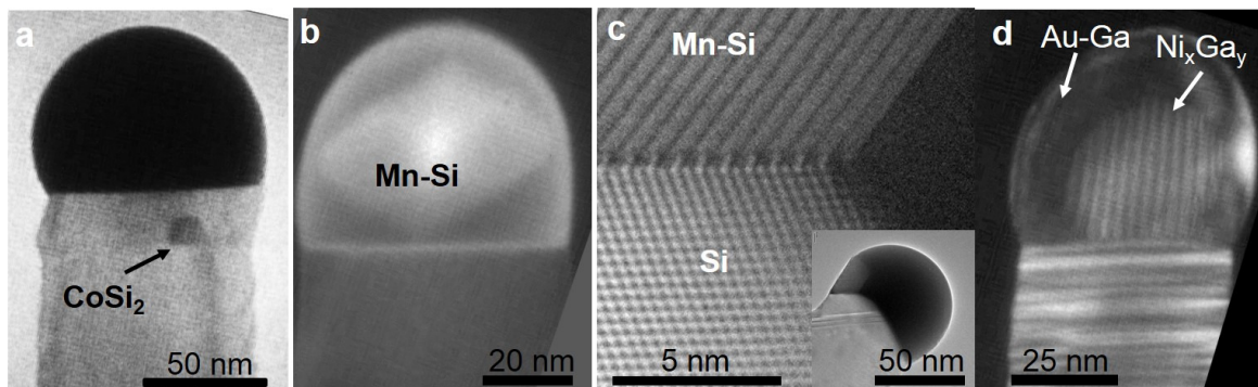
Figure 4: Nanocrystal formation in different materials. a \text{CoSi}_2 nanocrystal formed after 15 min of exposure to 5 \times 10^{-6} Torr of \text{Co}(\text{C}_5\text{H}_5)_2 at 500^\circ\text{C} and incorporated into a nanowire after switching to 5 \times 10^{-6} Torr of \text{Si}_2\text{H}_6 without changing temperature. The Si growth rate after \text{Co}(\text{C}_5\text{H}_5)_2 exposure was slower than expected, perhaps suggesting the presence of carbon on the catalyst surface; other metalorganic precursors are known to deposit less carbon at this temperature [31]. b MnSi nanocrystals formed after Mn evaporation onto the Au-Si catalyst. Similar results are obtained with gas precursor \text{Mn}(\text{C}_5\text{H}_5)_2 . c High resolution image of a Mn-Si nanoparticle in contact with the 111 surface of a nanowire, with the inset showing the whole nanowire. d A Ni-Ga nanocrystal formed in a liquid AuGa catalyst on a GaAs nanowire after 20 min exposure to 1 \times 10^{-6} Torr of \text{Ni}(\text{C}_5\text{H}_5)_2 at 500^\circ\text{C} ; image recorded after cooling.
