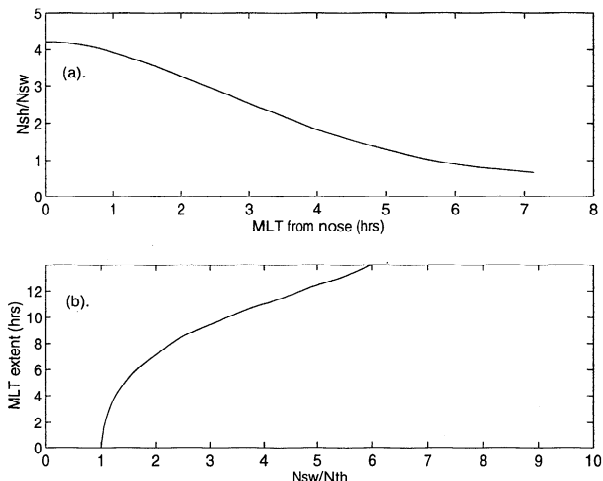
Figure 9. The prediction of the variation of cusp longitudinal extent as a function of solar wind density using the gas dynamic magnetosheath model of Spreiter et al. [1966]. (a) The ratio of magnetosheath density divided by the solar wind value, ( N_{sh}/N_{sw} ), as a function of the separation in MLT from the nose of the magnetosphere. (b) The MLT extent of that part of the magnetopause contributing to cusp precipitation region, as a function of N_{sw} , given as a ratio of its threshold value N_{th} (see text for details).
