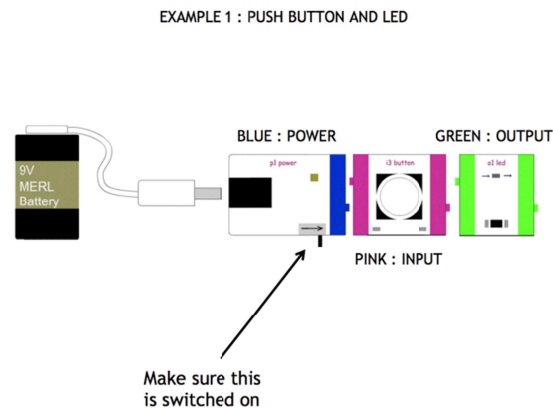
Figure 1: littleBits worksheet that describes how to construct a simple circuit containing a power source, button and LED.
