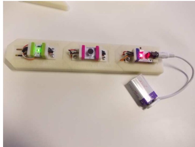
Figure 7: Top view of enlarged base for littleBits components, showing an LED control mounted on the base.
