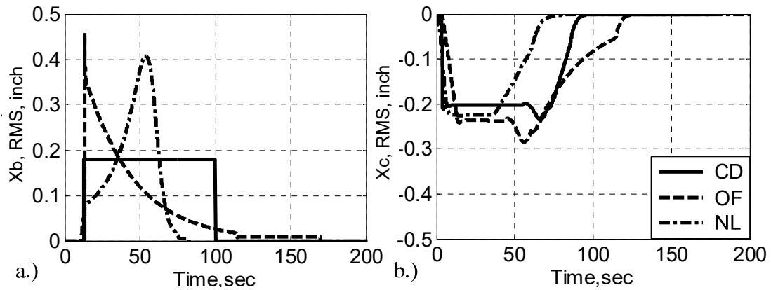
Fig. 19 Pilot model inputs for each of the designed profiles
