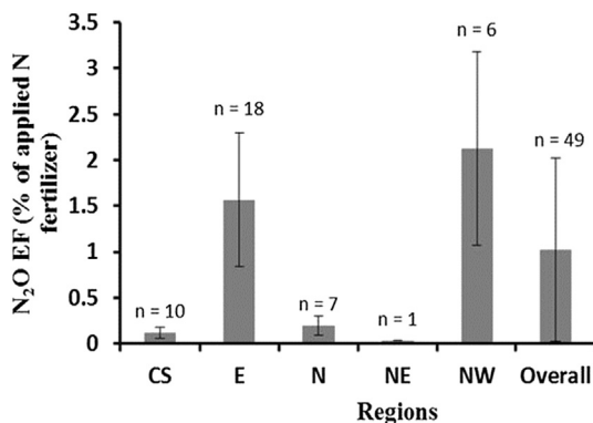
Fig. 4. Region specific N 2 O Emission Factors (EF) for wheat (transformed data). Abbreviation: CS – Central south including 4 provinces (Guangdong, Henan, Hubei, Hunan), E – East including 4 provinces (Jiangsu, Jiangxi, Shandong, Shanghai), N – North including 4 provinces (Beijing, Hebei, Inner Mongolia, Shanxi), NE – Northeast including 2 provinces (Heilongjiang, Liaoning), NW – Northwest including 1 province (Shaanxi).
