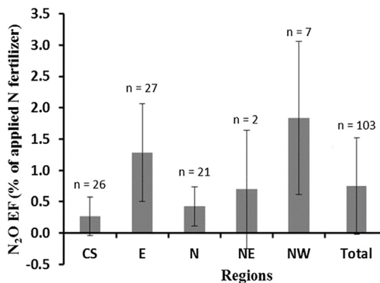
Fig. 3. Region specific N 2 O Emission Factors (EF) for upland crops (transformed data). Abbreviation: CS – Central south including 4 provinces (Guangdong, Henan, Hubei, Hunan), E – East including 4 provinces (Jiangsu, Jiangxi, Shandong, Shanghai), N – North including 4 provinces (Beijing, Hebei, Inner Mongolia, Shanxi), NE – Northeast including 2 provinces (Heilongjiang, Liaoning), NW – Northwest including 1 province (Shaanxi).
