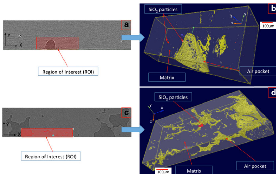
Fig. 9 (a) X\mu CT reconstruction of binary image of 10% loaded sample with selected Region of Interest (ROI) for analysis; (b) 3D object representing the different components according to their densities present in the selected ROI; (c) X\mu CT reconstruction of binary image of 20% loaded patches with selected Region of Interest (ROI) for analysis; (d) 3D object representing the different components according to their densities present in the selected ROI.
