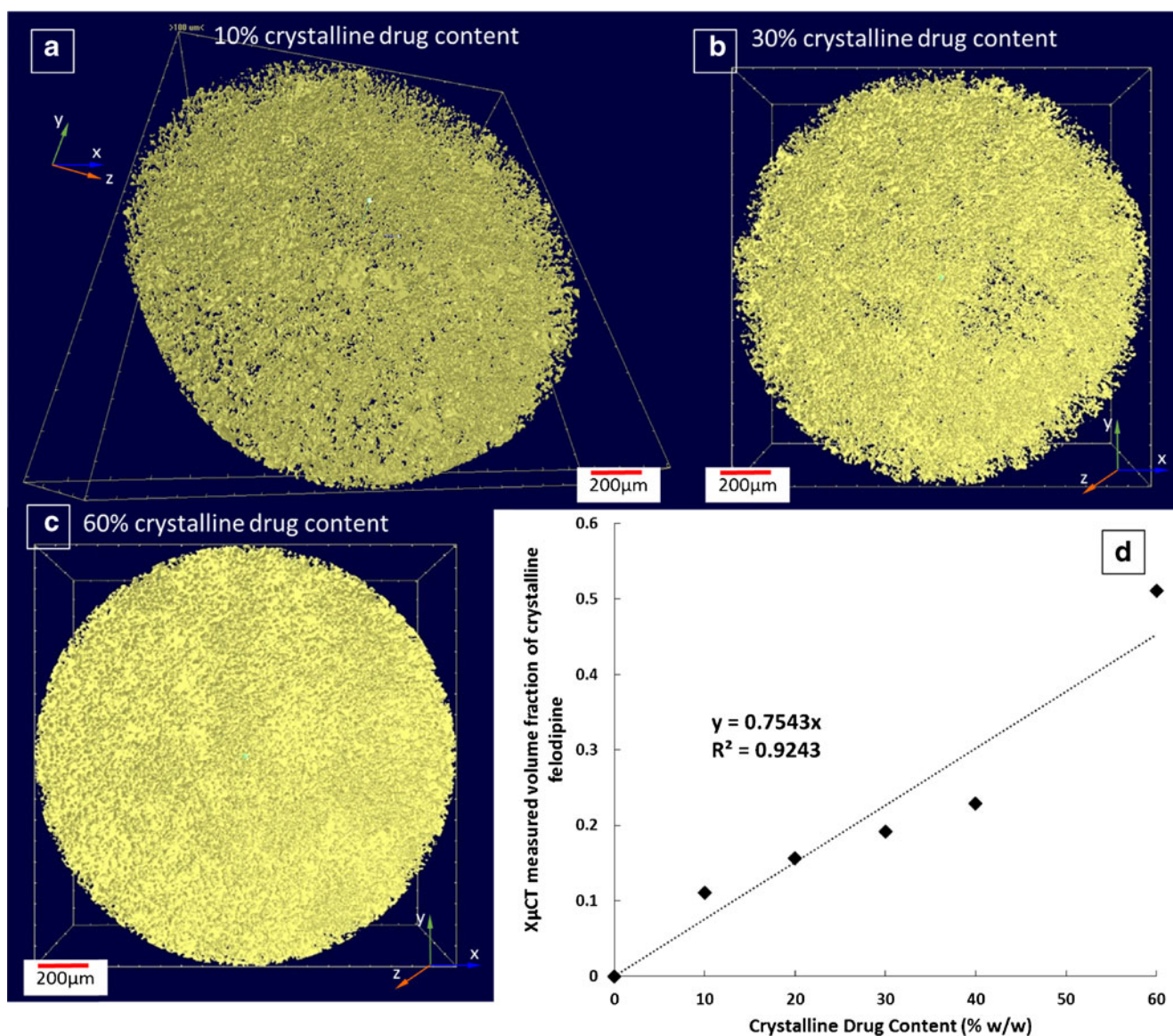
Fig. 11 Representative 3D X \mu CT images of the distribution of crystalline felodipine in the compacts made of the physical mixes of crystalline felodipine-TPGS-PEG-PEO with (a) 10%; (b) 30%; and (c) 60% crystalline felodipine loadings. (d) the correlation between crystalline drug content in these compacts and measured volume fraction of felodipine in their 3D X \mu CT images, which was used as calibration curve for the quantitative estimation of crystalline felodipine in HME-IM patches with 30% drug loading.
