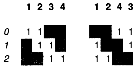
Figure A.4 The path \pi(2, 4)
