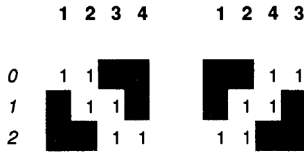
Figure A.3 The path \pi(2, 1)
