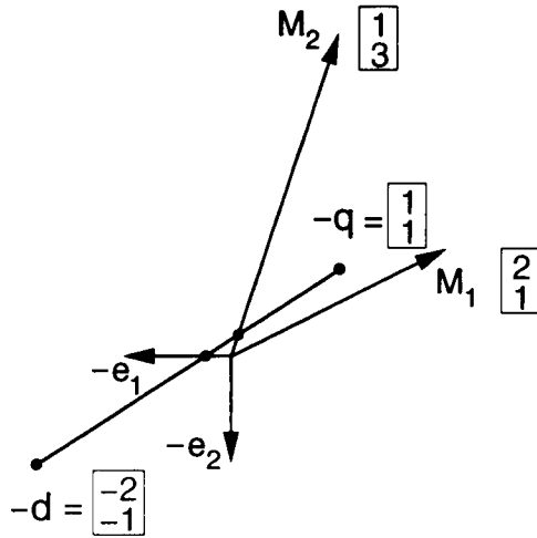
Figure 4.4 Lemke’s algorithm as inverting the piecewise linear LCP map F along the line segment [-d, -q] . The computation involves four basic solutions, corresponding to the endpoints -d and -q , and the facets of the complementary cones that the line segment crosses. Thus, the computation involves three pivoting steps.
