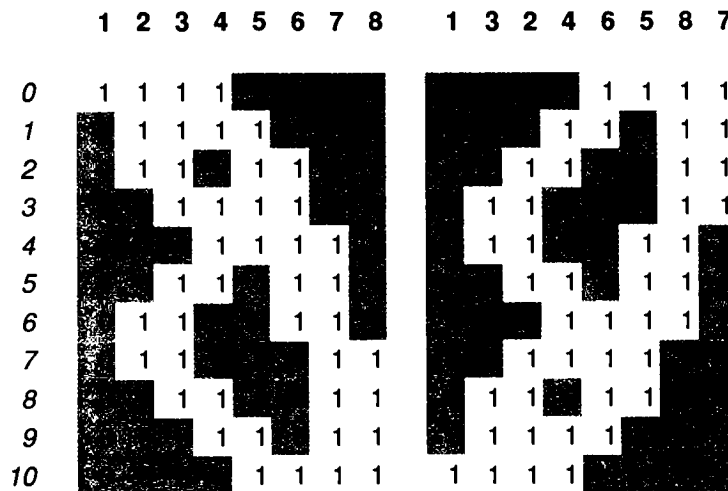
Figure A.5 The path \pi(4, 1)
