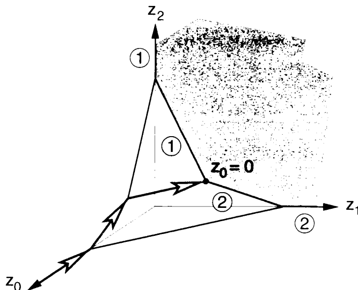
Figure 4.2 An illustration of Lemke's algorithm
