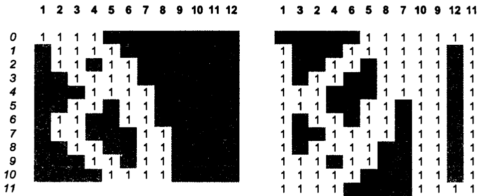
Figure A.16 The path \rho(4, 12)
