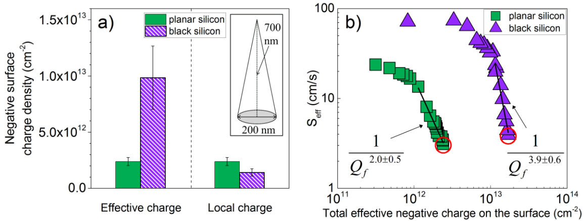
Figure 5: a) Average \text{Al}_2\text{O}_3 charge density measured on planar and black silicon samples passivated with 20 nm of \text{Al}_2\text{O}_3 . An effective charge density is seen at the macroscopic scale. The local charge density was obtained by taking into account the surface area enlargement in black silicon. The inset presents a schematic of a typical b-Si needle. b) Maximum surface recombination velocity as a function of the total negative charge after corona charging on both sides of the samples. The total charge corresponds to the sum of the corona charge and of the built-in \text{Al}_2\text{O}_3 charge, and the circles show the initial measurement points before Corona charging.
