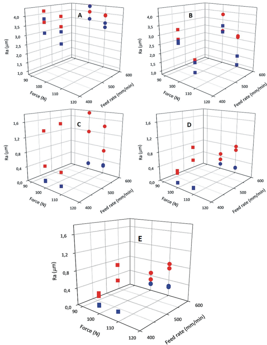
FIGURE 5.—Influence of the parameters on the surface roughness in A92017 workpieces. A- R_a // 1pass. B- R_a // 5passes. C- R_a \perp 1pass. D- R_a \perp 5passes. Blue: vibration-assisted-burnishing; Red: non-vibration-assisted-burnishing; Circles: f = 600 mm/min; Squares: f = 400 mm/min. E- Comparison between conventional burnishing process and vibration-assisted-burnishing for the same system parameters ( f , F and n ). Blue: vibration-assisted burnishing, 1pass. Red: non-vibration-assisted burnishing, 5passes.
