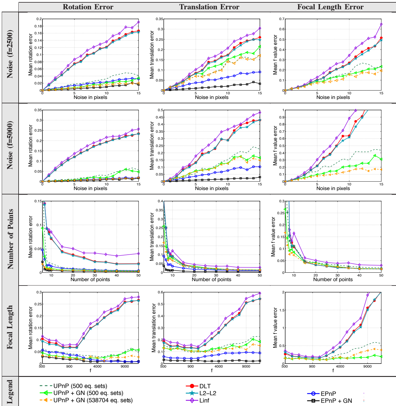
Fig. 5. Results on synthetic data for non-planar distributions of points. Two upper rows: Mean rotation, translation and focal length errors for: increasing levels of image noise on 10 2D-3D correspondences, and two different focal lengths. Third row: increasing number of 2D-3D correspondences. Fourth row: increasing focal length, also for 10 point correspondences. Each tick in the plot represents the average over 100 experiments with random points.
