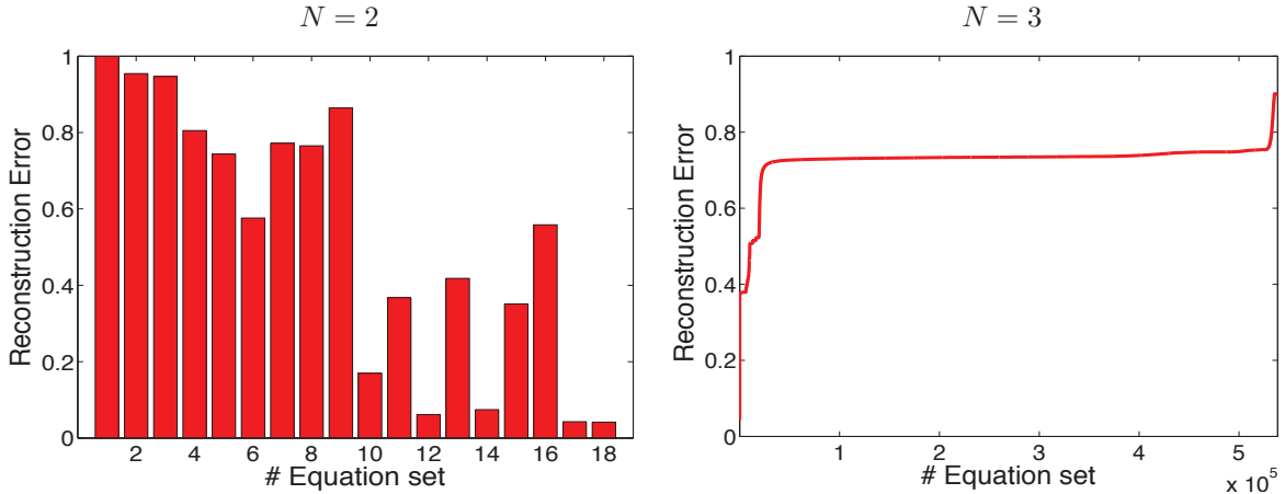
Fig. 2. Reconstruction error for all possible equation sets. The graphs plot the mean normalized reconstruction error over 1000 different experiments with random input correspondences, and different amounts of noise. Left. All 18 triplet combinations for a kernel of size N = 2 . Right. All 538.704 quadruplet combinations for a kernel of size N = 3 . In this case, the reconstruction errors have been sorted in increasing order of magnitude for viewing purposes. Observe that in both cases, the selection of one set of equations from another, results in significantly different reconstruction error (and hence pose and focal length estimation).
