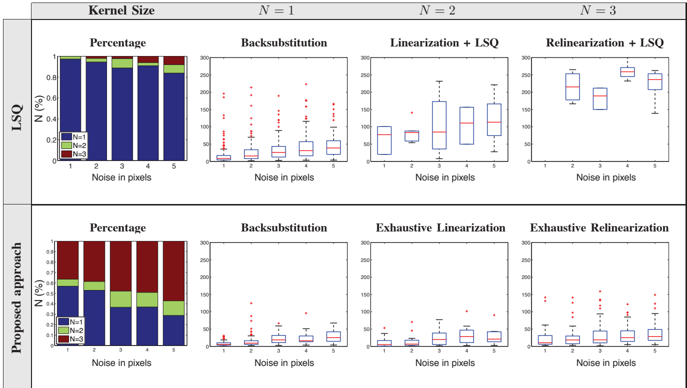
Fig. 3. Comparison of our approach that estimates the parameters via backsubstitution over minimal equation sets, against an approach that estimates these via backsubstitution over a least squares approximation using all equations for a set of 1000 experiments and varying image noise. Left column: Effective number N of null eigenvalues of M^T M . Second to fourth columns: Reprojection error distributions (in pixels) for the N = 1 , N = 2 , and N = 3 cases. The box edges in the boxplots denote first and third quartiles, red lines inside the boxes indicate medians, dashed lines represent the extent of the statistical data, and red crosses are outliers.
