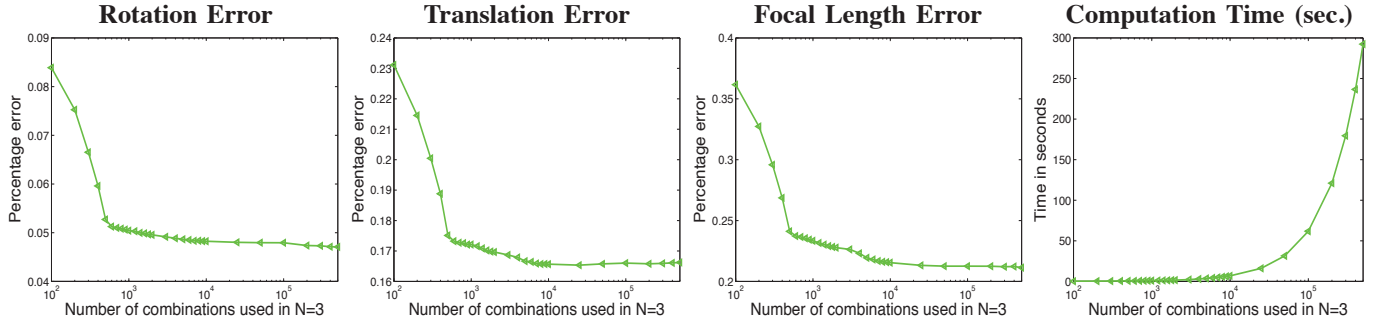
Fig. 4. Mean rotation, translation and focal length estimation errors when N = 3 is selected as the best solution (we refer the reader to Sec. 4.1 for a precise definition of these errors), and computation time for an increasing number of equation sets. Note that the horizontal axis is plotted in logarithmic scale, and the time scales linearly with the number of equation sets. Exploring 500 equation sets is a good trade off between accuracy and computation time. These graphs are generated with random experiments with n = 7 points, and large amounts of 2D noise (at the level of \sigma_n = 5 ), in order to ensure that exploration of the case N = 3 was meaningful.
