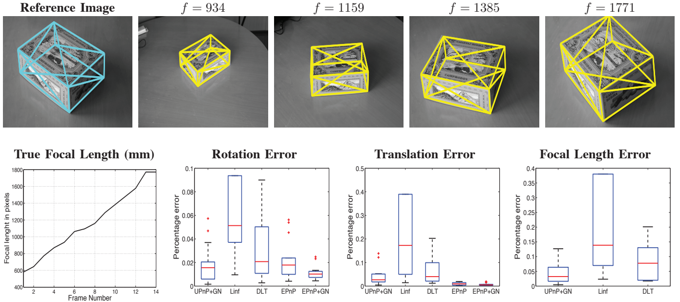
Fig. 8. Results on a real sequence with increasing focal length. Top. 3D model reprojected onto the reference and input images using the pose and focal length retrieved with the UPnP. Bottom. Ground truth focal length and performance comparison of all methods.
