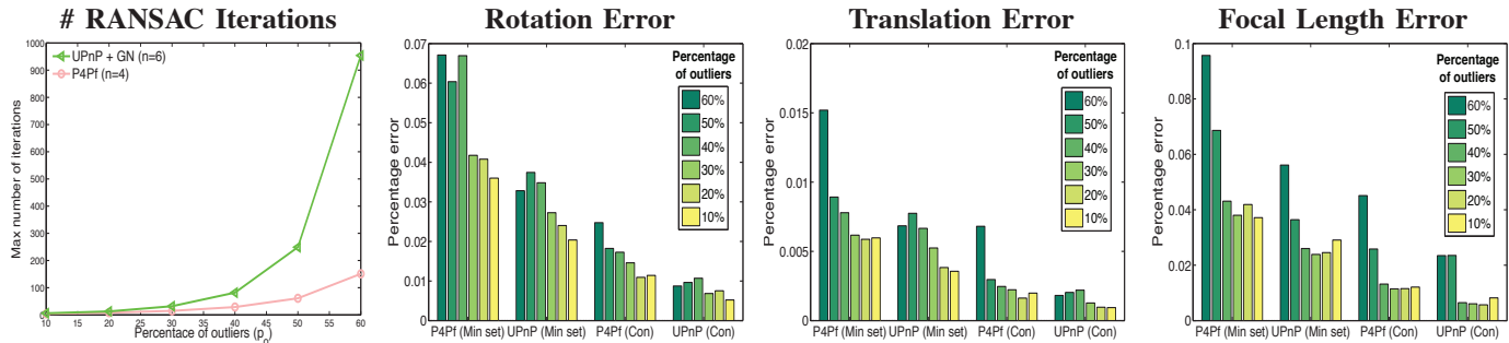
Fig. 11. Comparison of UPnP vs P4Pf within a RANSAC scheme. Left: Number of iterations required to retrieve a hypothesis of n point correspondences free of outliers, where n = 4 for the P4Pf and n = 6 for the UPnP. Other three frames: Rotation, Translation, and Focal length errors for different levels of outliers. Min set: Errors obtained when computing pose using the best minimal subset. Con: Error after computing pose using all the correspondences within the inlier set. Since the P4Pf does not generalize to more than four correspondences, the error of the consensus is computed using the UPnP in both cases.
