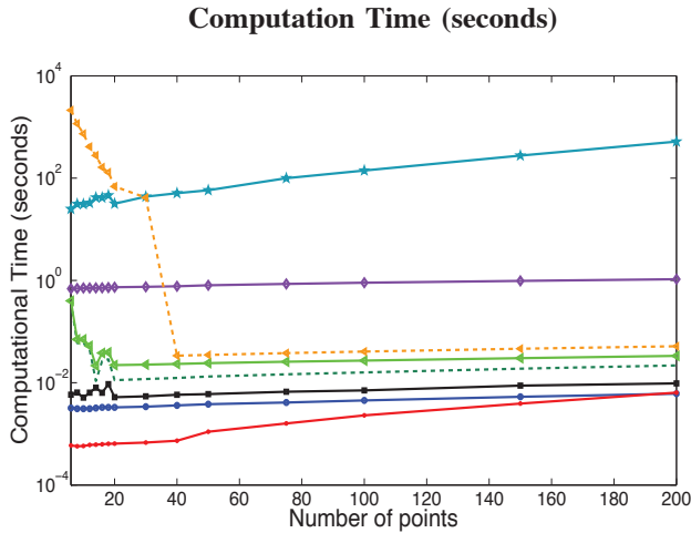
Fig. 6. Comparison of the computation time of our method against state of the art approaches with respect to the number of input points, and for fixed values of f = 2500 and \sigma_n = 5 . The color codes and line styles are the same as those used in Fig. 5.
