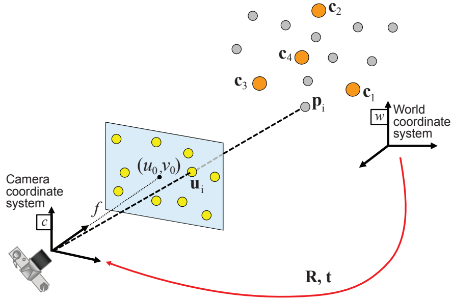
Fig. 1. Problem Formulation: Given a set of correspondences between 3D points \mathbf{p}_i expressed in a world reference frame, and their 2D projections \mathbf{u}_i onto the image, we seek to retrieve the pose ( \mathbf{R} and \mathbf{t} ) of the camera w.r.t. the world and the focal length f .
