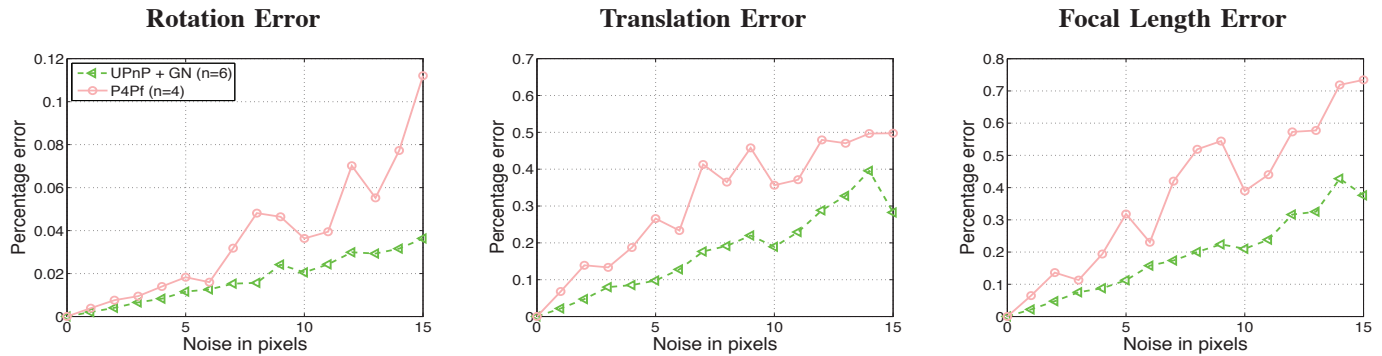
Fig. 10. Comparison of the UPnP using 6 correspondences vs. the minimal approach proposed in [2], which estimates pose and focal length from four 3D-to-2D correspondences.
