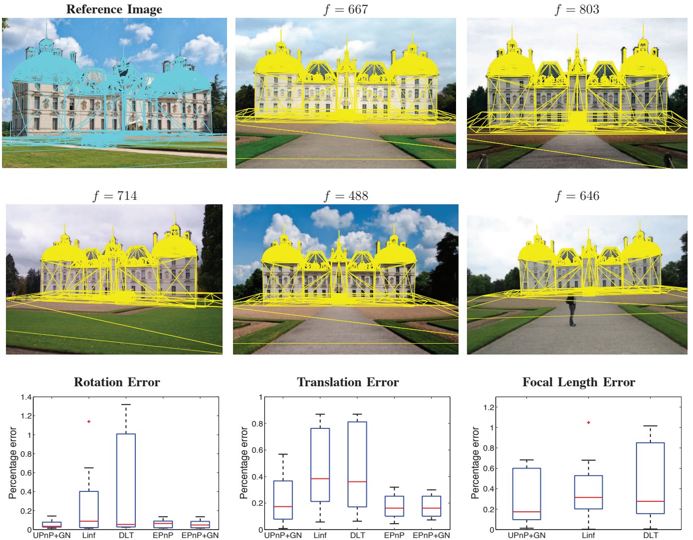
Fig. 9. Results on a real set of images obtained from Flickr with a 3D model obtained from GoogleEarth . Top. 3D model reprojected onto the reference and input images using the pose and focal length retrieved with the UPnP . Bottom. Comparing the accuracy of our approach against Linf, DLT, EPnP and EPnP+GN. The last two methods assume a calibrated camera.
