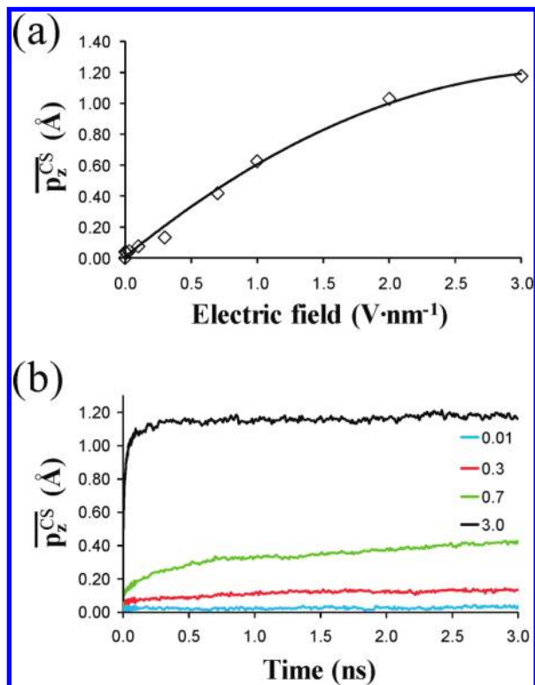
Figure 5. (a) Variation of the temporal average value of the averaged projection of the C–S bond into the z -axis ( p_z^{\text{CS}} ) against the electric field. (b) Temporal evolution of p_z^{\text{CS}} for selected electric fields, which are represented using different colors.
