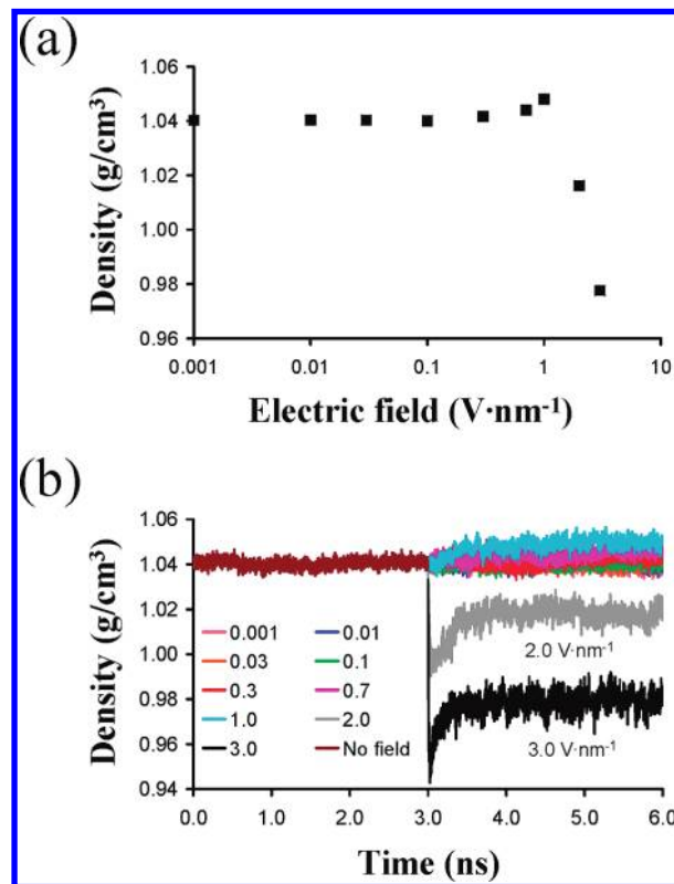
Figure 4. (a) Variation of the average density against the electric field and (b) temporal evolution of the density obtained considering E_z = 0.001, 0.01, 0.03, 0.1, 0.3, 0.7, 1.0, 2.0, and 3.0 \text{ V}\cdot\text{nm}^{-1} .
