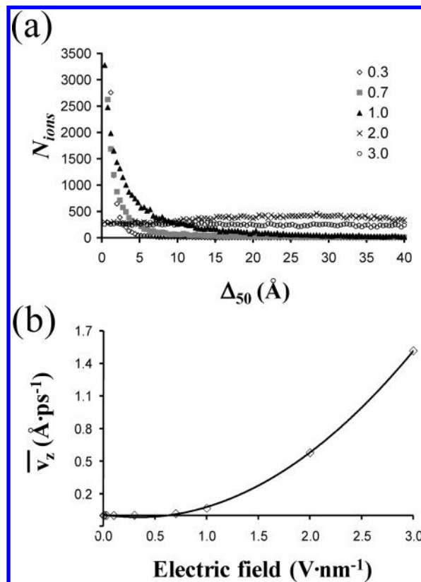
Figure 6. (a) For selected electric fields, variation of the number of hydronium ions ( N_{\text{ions}} ) against the distance covered in the simulation box during 50 ps ( \Delta_{50} ) when \Delta_{50} \geq 0.4 \text{ \AA} . (b) Variation of the average velocity of the hydronium ions along the z -axis ( V_z ) against the electric field.
