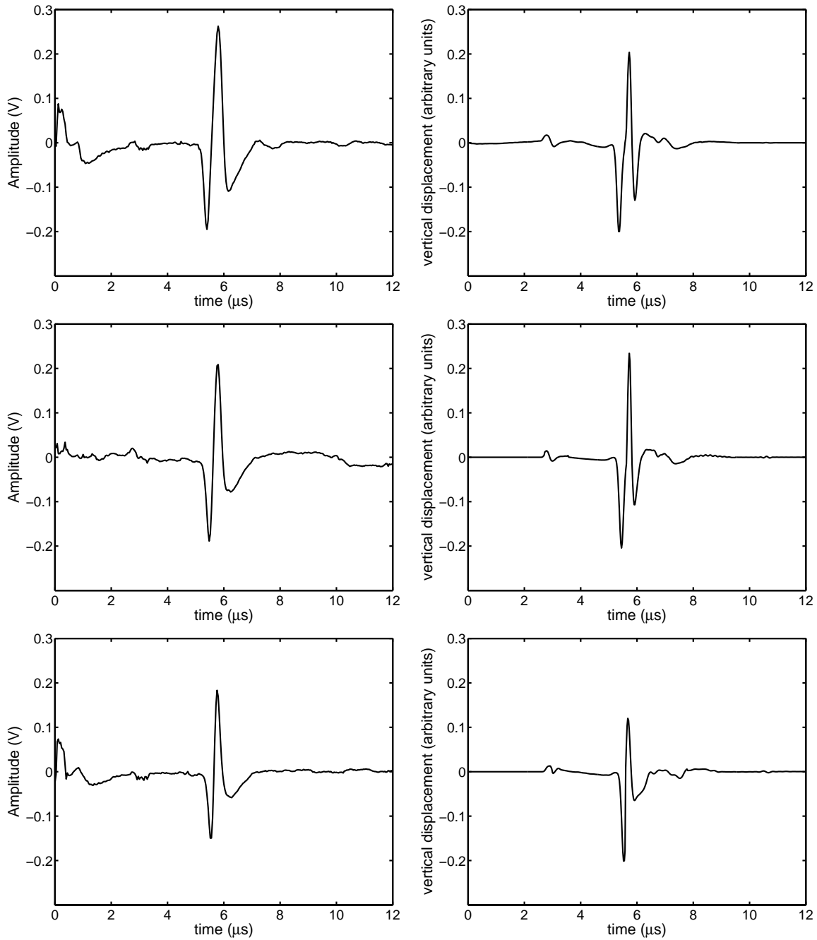
Fig. 9. Experimental (left column) and simulated (right column) signals at the receiver when the laser is located at distances of 0.75, 0.5 and 0.25 mm from the left face of the notch.
