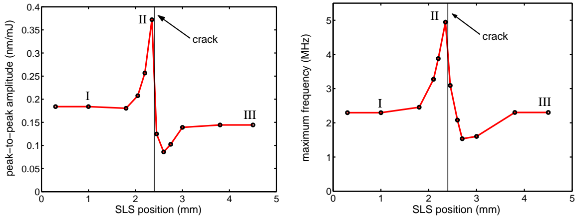
Fig. 13. Simulated signatures of the defect in the ultrasonic amplitude (left) and the maximum frequency (right) of the generated signal as the laser source scans over a surface-breaking crack.
