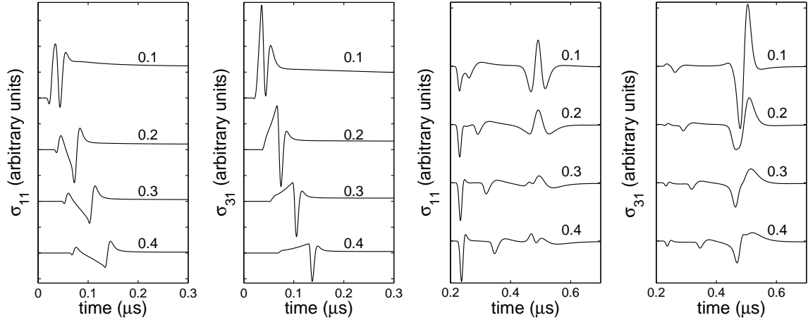
Fig. 5. Tractions on the vertical plane at 0.05 mm (left) and 1.4 mm (right) distance from the axis of the laser line-source at various depths. The numbers next to the waveforms indicate the depth in mm. A negative normal traction indicates compression and a positive shear traction on the top face of an element points in the negative x_1 direction.
