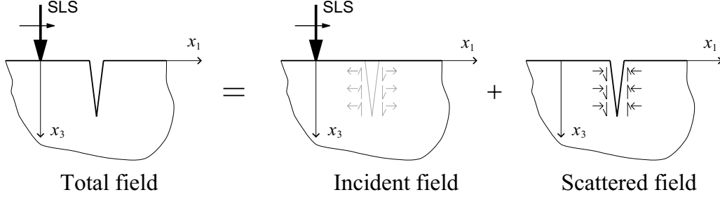
Fig. 2. Decomposition of the total field into incident and scattered fields.
