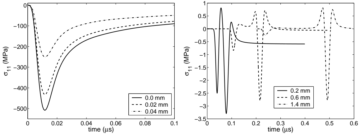
Fig. 4. Stress component \sigma_{11} on the surface. The legend indicates the distance to the epicentral axis. A negative value of \sigma_{11} indicates compression.
