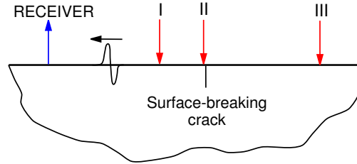
Fig. 11. Configuration for the SLS technique. Three positions of the laser line-source (I,II, and III) are displayed.
