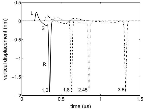
Fig. 3. Normal displacement on the surface. The numbers next to the waveforms indicate the distance in mm from the axis of the laser line-source. The labels L, S and R denote longitudinal, shear and Rayleigh surface waves, respectively. A negative value represents an inward normal displacement.
