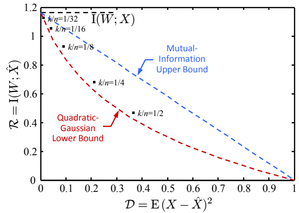
Fig. 9: Privacy-distortion performance of \mu -Approx on scalar data.
