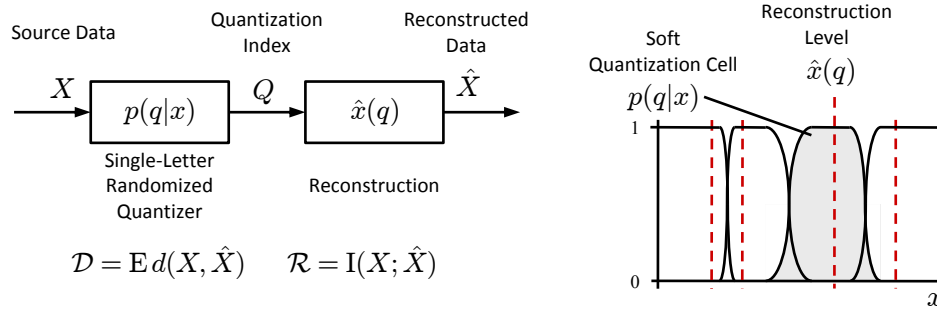
Fig. 4: Single-letter characterization of the rate-distortion problem.
