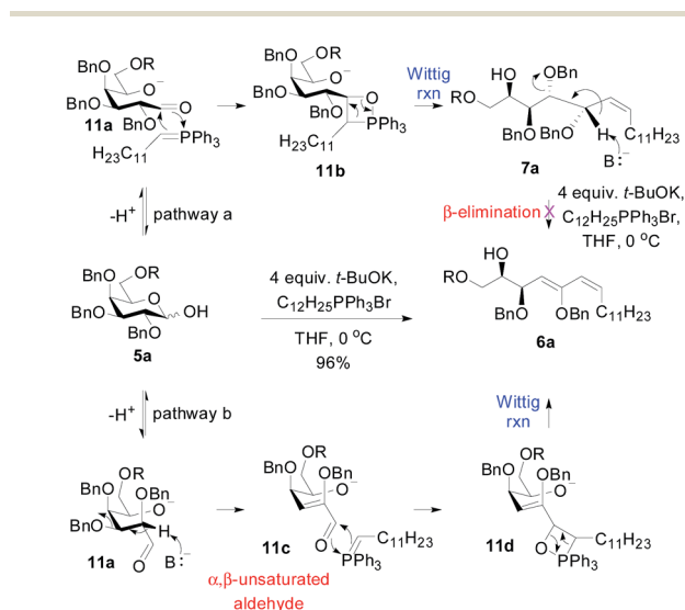
Scheme 1 Plausible mechanism of unusual Wittig reaction.
