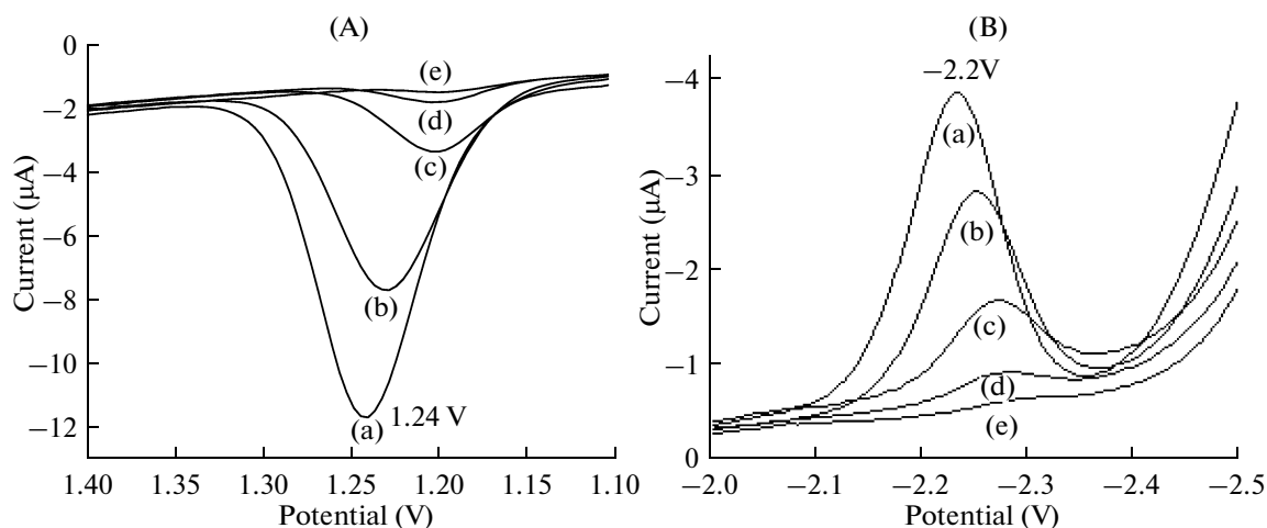
Fig. 2. DPV voltammograms of carbamazepine under optimum conditions: (a) 2.0 \times 10^{-4} M; (b) 1.0 \times 10^{-4} M; (c) 4.0 \times 10^{-5} M; (d) 1.0 \times 10^{-5} M; (e) 1.0 \times 10^{-6} M at +1.24 V (A) and -2.2 V (B).
