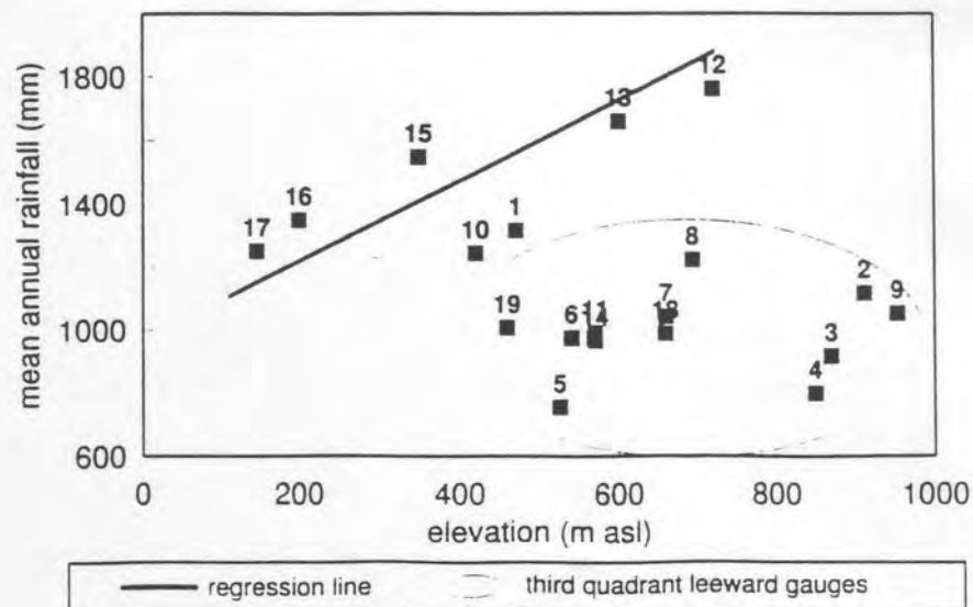
Figure 3 Long duration gauge elevation plotted against rainfall
