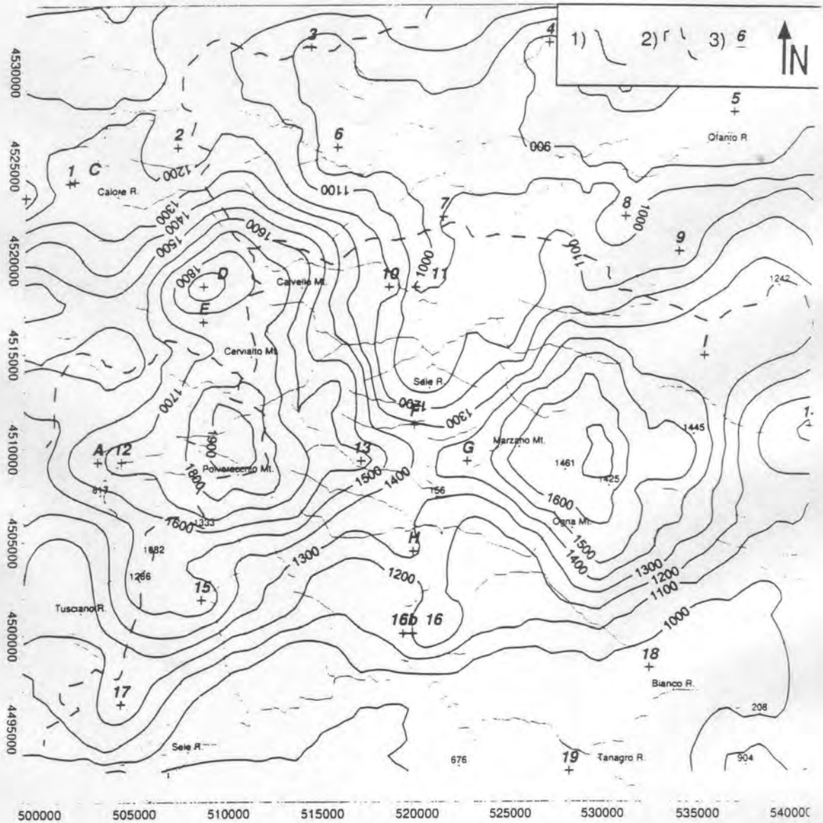
Figure 4 Mean yearly rainfall map: (1) isohyet (mm); (2) drainage divide; (3) gauge.
