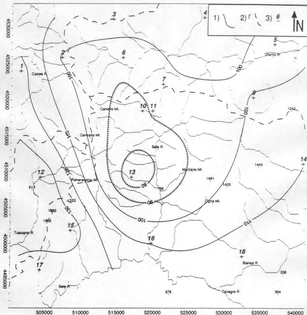
Figure 6 Total rainfall over the 12 months before the 1980 earthquake, expressed as percentage of the historical mean: (1) isohyet (%); (2) drainage divide; (3) gauge.
