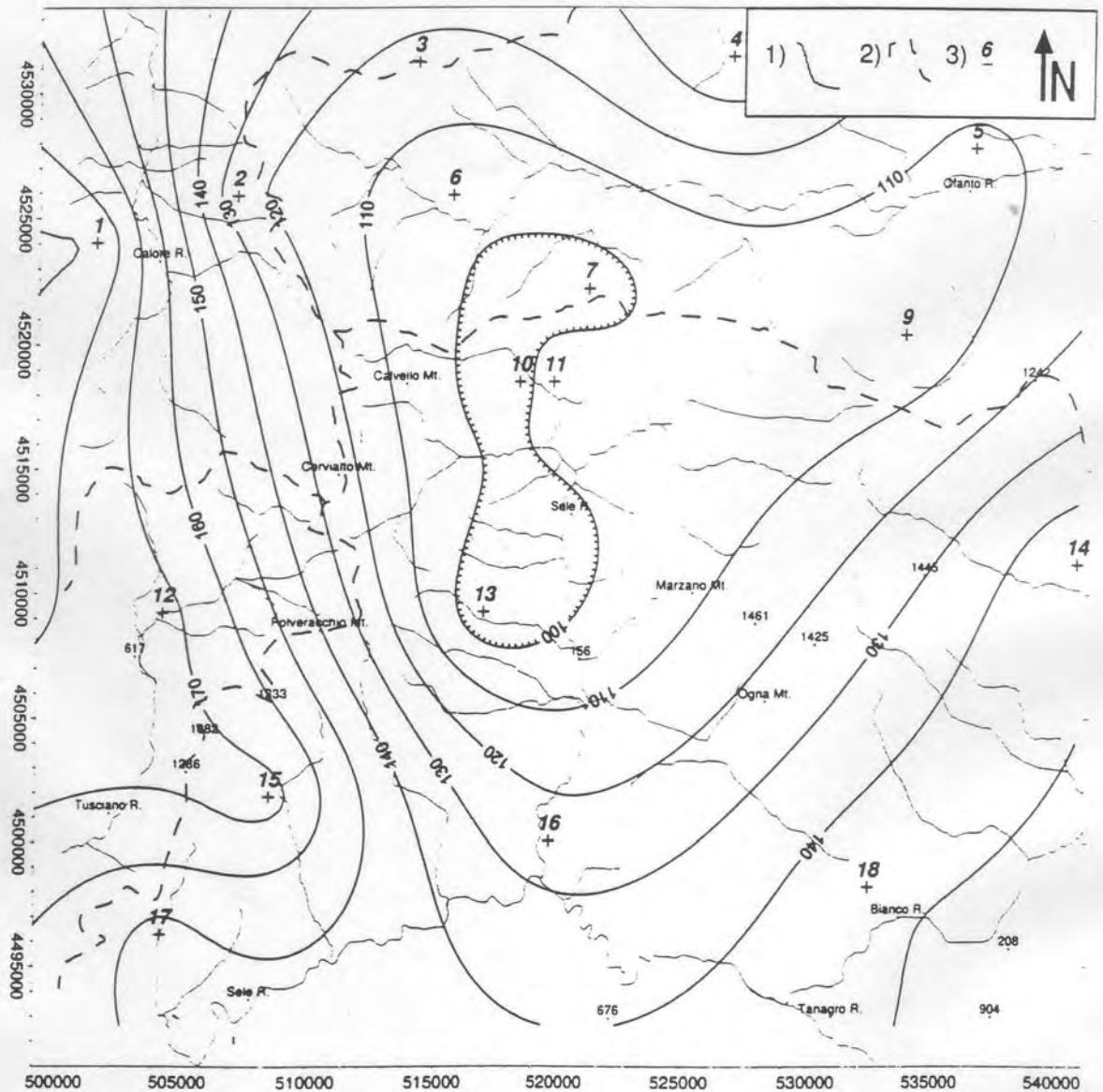
Figure 5 Total rainfall over the three months before the 1980 earthquake, expressed as a percentage of the historical mean: (1) isohyet (%); (2) drainage divide; (3) gauge.
