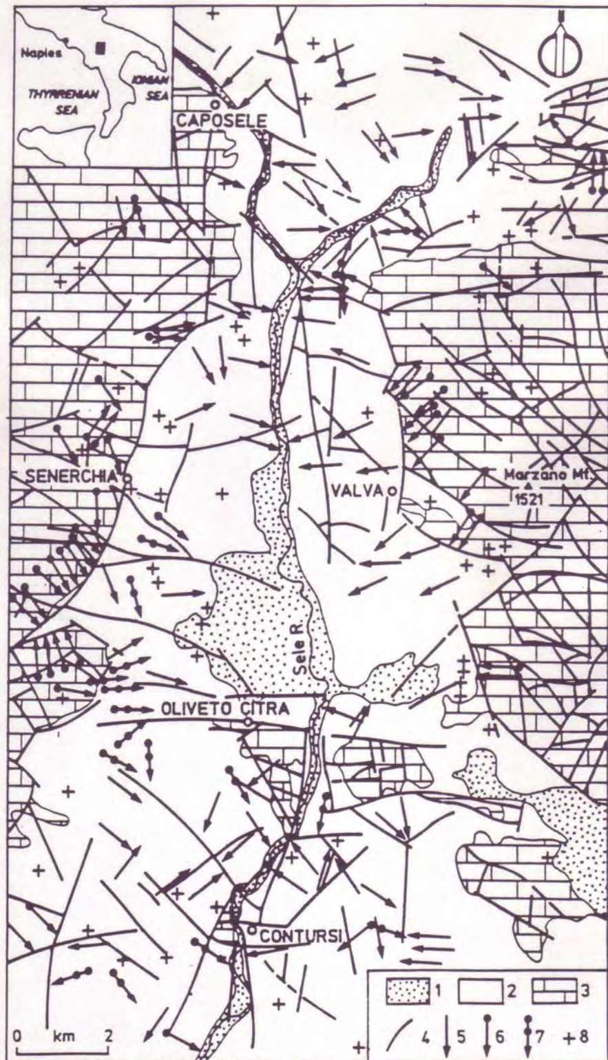
Figure 1 Schematic map of the geology, hydrogeology and morphology of landslides (after Agnesi et al. , 1982; Polemio, 1997): (1) alluvial deposits, medium relative primary permeability; (2) clayey-marly flysch with calcareous, arenaceous or calcareous-marly interbeds or blocks, very low to low relative primary permeability, medium secondary permeability; (3) limestone, dolomitic limestone, dolomite, of medium to very high relative secondary permeability due to fracturing and karstification; (4) landslides before 1980; (5) landslides since the 1980 earthquake; (6) type 4 and 5 landslides; (7) fault; (8) spring.
