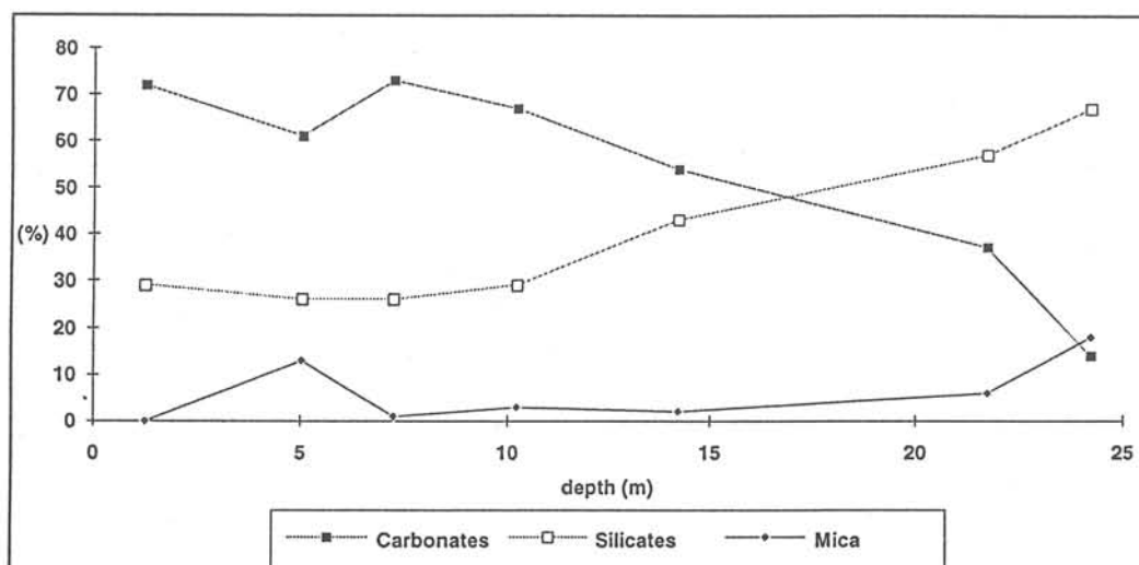
Fig. 3. Mineralogical composition variations with depth
