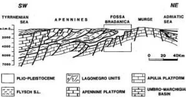
Figure 2: Schematic geological map and geological section of the southern Apennines (after Sella et al., 1988).
