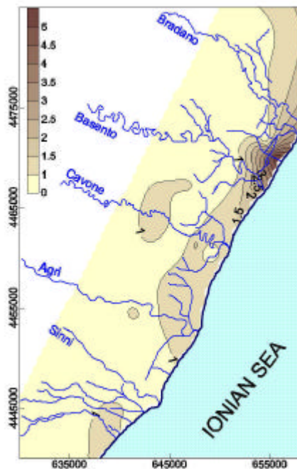
Figure 11: Map of characteristic ratio (Na + + K + + Cl - + SO 4 2- )/(Ca 2+ + Mg 2+ + HCO 3 - ) (as epm ratio).
