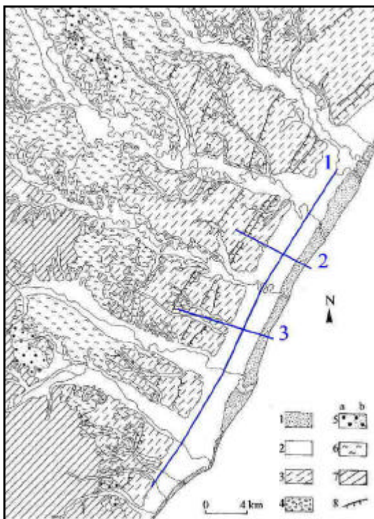
Figure 3: Schematic geological map of the study area: 1) coastal deposits; 2) alluvial, transitional and marine deposits; 3) marine terraces; 4) Conglomerato di Irsina Formation; 5) Sabbie di Monte Marano Formation (a) and Sabbie di Tursi Formation (b); 6) Argille subappennine Formation; 7) allochthon; 8) marine terraced scarps; the lines of the lithological sections in Figure 4 are reported.
