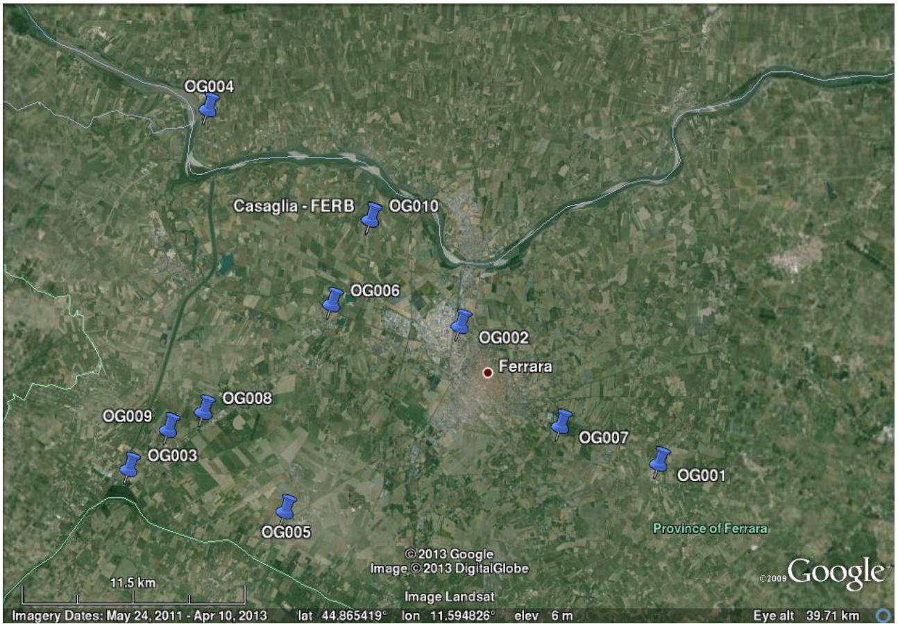
Fig. 1: OGS Temporary Network deployed in Ferrara area. Site OG010 is set at the top of the borehole hosting the FERB station. Site OG012 is very close OG002.
