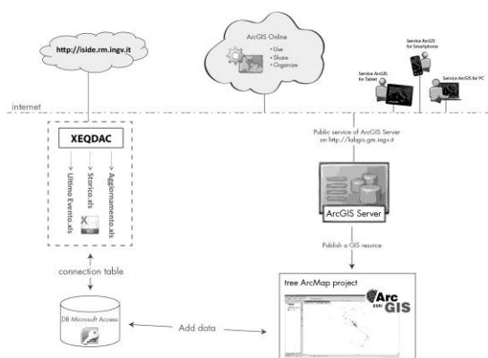
Figure 2 – The XEQDAC workflow
