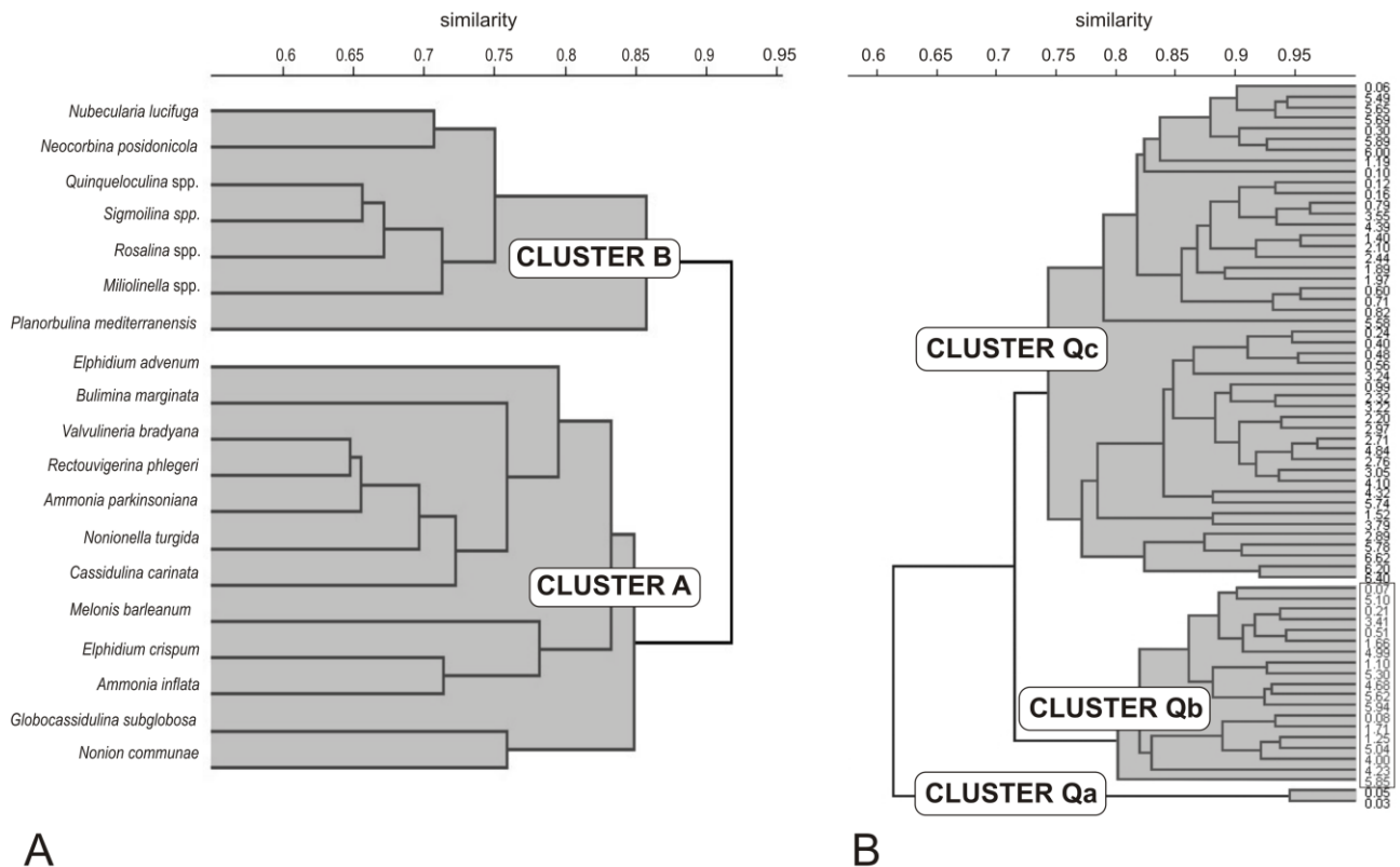
Fig. 3. Dendrogram classifications resulting from multivariate cluster analysis based on the relative abundance of the 19 most common benthic foraminifera taxa. A) Foraminiferal assemblage produced by R-mode analysis using Horn's (1966) modified version of Morisita's (1959) index; B) Sample associations produced by the Q-mode analysis performed with a Morisita's distance. Cluster B is well correlative of Cluster Qb and concur in the definition of 11 anomalies in the core.
