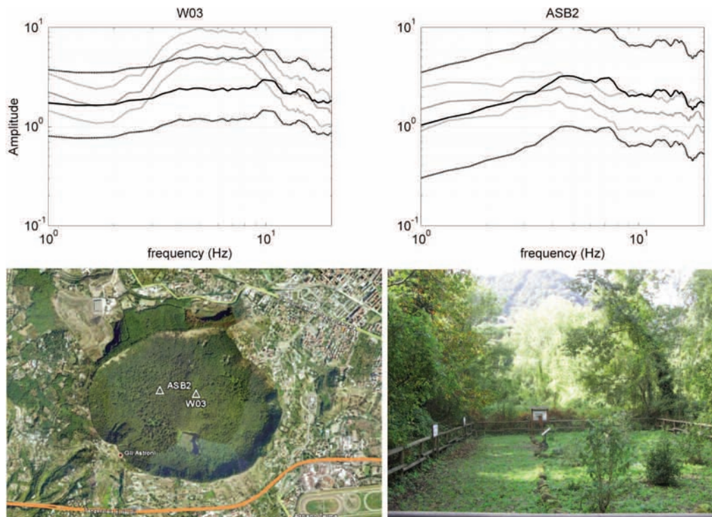
Figure 8 In the top panels we show the site transfer functions obtained with the H/V method (grey) and with the generalized inversion technique (black) for the station W03 (left) and for the station ASB2 (right). The upper and lower lines show the 1\sigma error. The bottom panels show the Google Earth image of the stations W03 and ASB2 (left) and a picture of the place where the station ASB2 is deployed (right).
