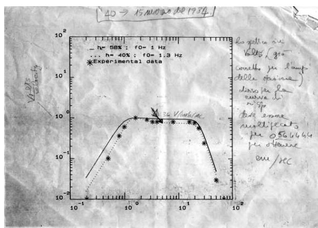
Figure 2 Data sheet of the 1984 reporting the transfer function of the Wisconsin Network sensors.
