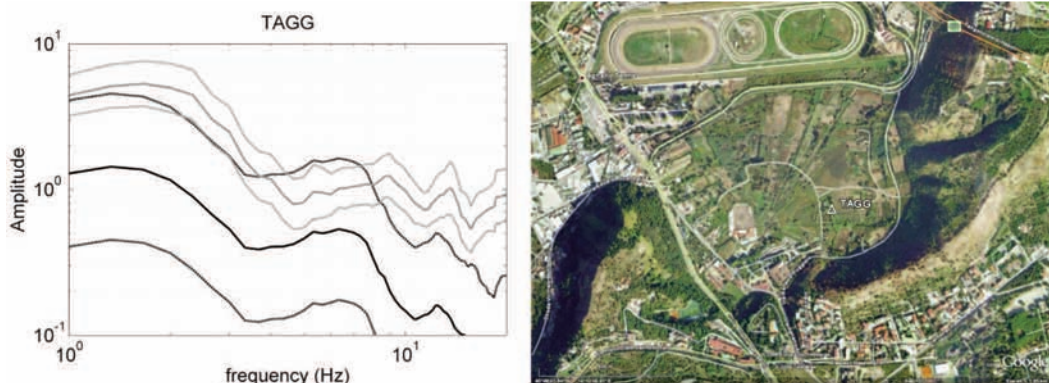
Figure 10 In the left panel we show the site transfer functions obtained with the H/V method (grey) and with the generalized inversion technique (black) for the station TAGG. The upper and lower lines show the 1 \sigma error. The right panel show the Google Earth image of the station TAGG.
