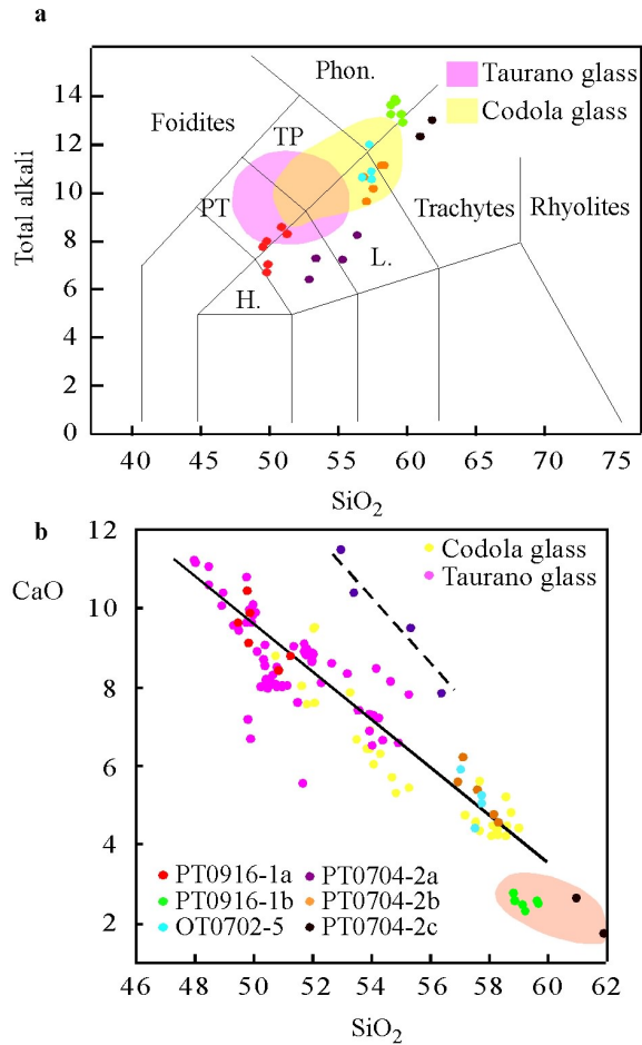
Fig. 6. (a) Total alkali vs. silica diagram for the different groups of OT0702-5 (pale blue dots), PT09-16 (red and green dots), PT0704-2 (purple, orange and black dots); (b) CaO vs. \text{SiO}_2 diagram for the same groups of Fig. 5a.
