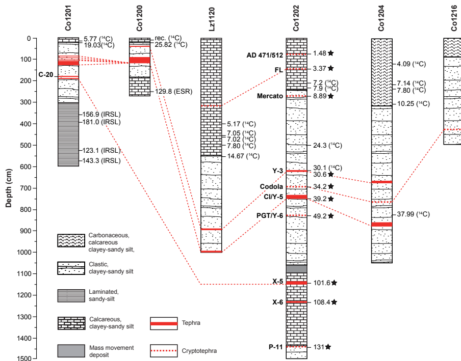
Fig. 2. Summary of stratigraphy and lithology of the studied cores. The thicknesses and sediment depths of tephras and cryptotephra are indicated by red horizons. Dashed lines between the cores indicate the correlation of individual tephras and cryptotephra. Age control for the different sediment successions apart from tephrochronology is given by radiocarbon ( 14 C), infrared stimulated luminescence (IRSL), and electron spin resonance (ESR) dating.
