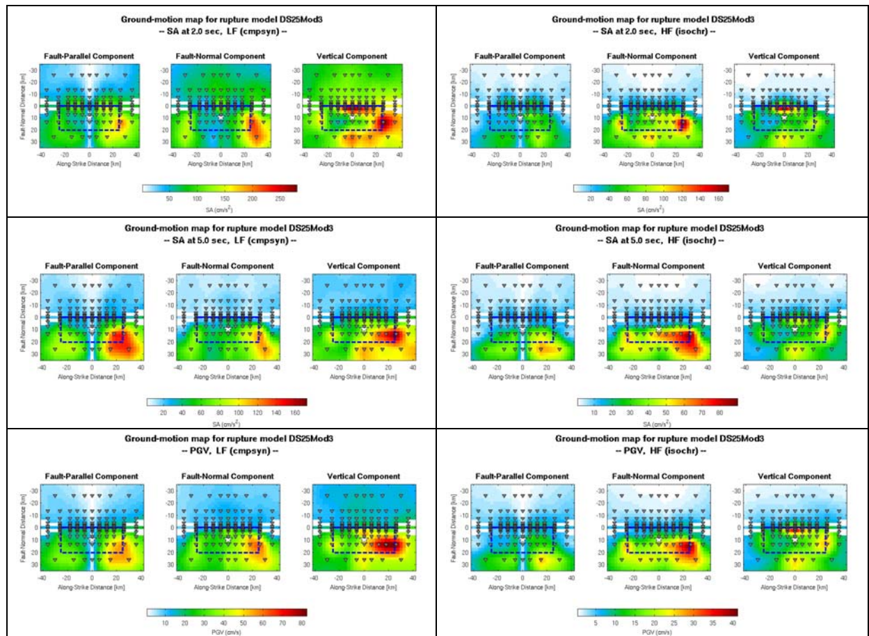
Figure 8. Shake maps for 25^\circ dipping thrust-faulting scenario event DS25Mod3 for T = 2\text{sec} (top row), T = 5\text{sec} (center row) and PGV (bottom row), for full-wave field (left column) and far-field (right column) synthetics. For details see Figure 7. Note the similarities in the overall shaking pattern between the two sets of synthetics, but also the differences in the details (particularly in the vertical component and for the footwall stations) due to near-field effects.
