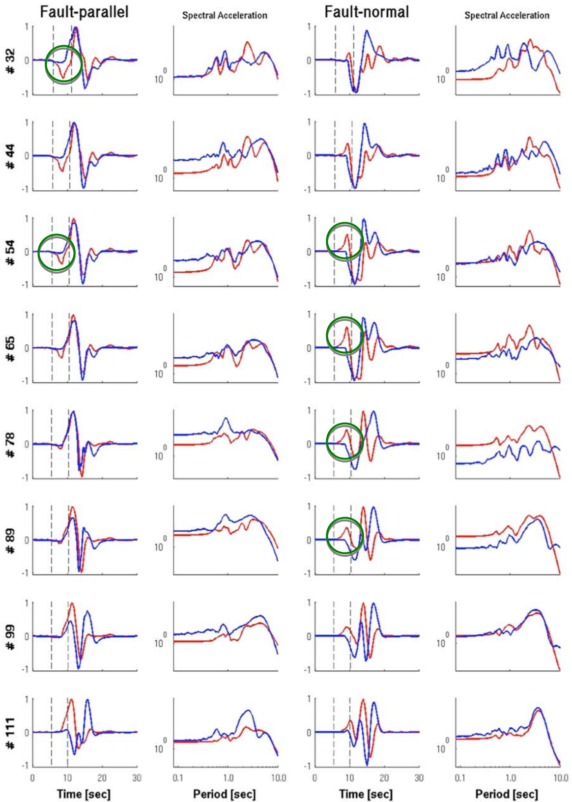
Figure 6. Same as Figure 5, for rupture models DS45Mod3.
