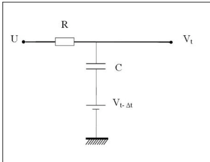
Figure 2. Sketch of an RC circuit. The initial charge of the capacitor C is represented by the cell V_{t-\Delta t} . U is the input signal while V_t is the filtered output at time t .
