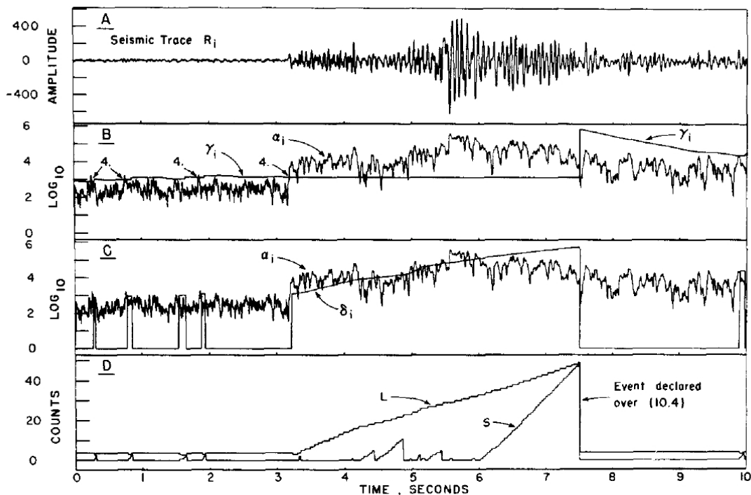
FIG. 4. Operating parameters during an event. (a) Seismic trace. (b) Short-term average \alpha_i , of characteristic function and reference level, \gamma_i . Points indicated as "4" refer to statement 4 in program flow charts. Note false onsets before arrival of real event. Amplitude scale is logarithmic. (c) Short-term average \alpha_i , and the criteria level \delta_i , carried during observation of an event. Logarithmic amplitude scale. (d) Quantities L and S, which determine point at which event is declared over.
