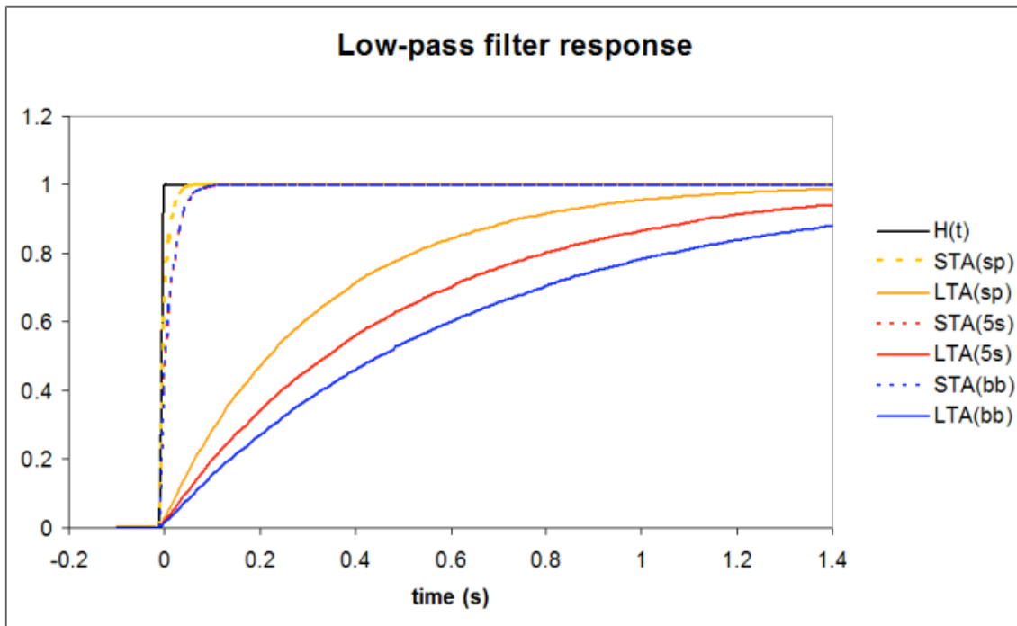
Figure 3. Responses of the low-pass filters (proposed in this report) to an Heaviside input function.
