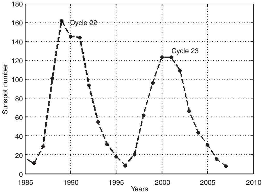
Fig. 4. Yearly average Sunspot number in the time interval 1985-2007.
