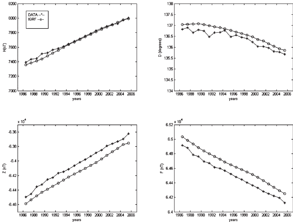
Fig. 3. Long-term time evolution of the H, D, Z and F elements at Mario Zucchelli Station, shown by their summer mean values (stars) and corresponding IGRF values (circles) (1986-2006).
