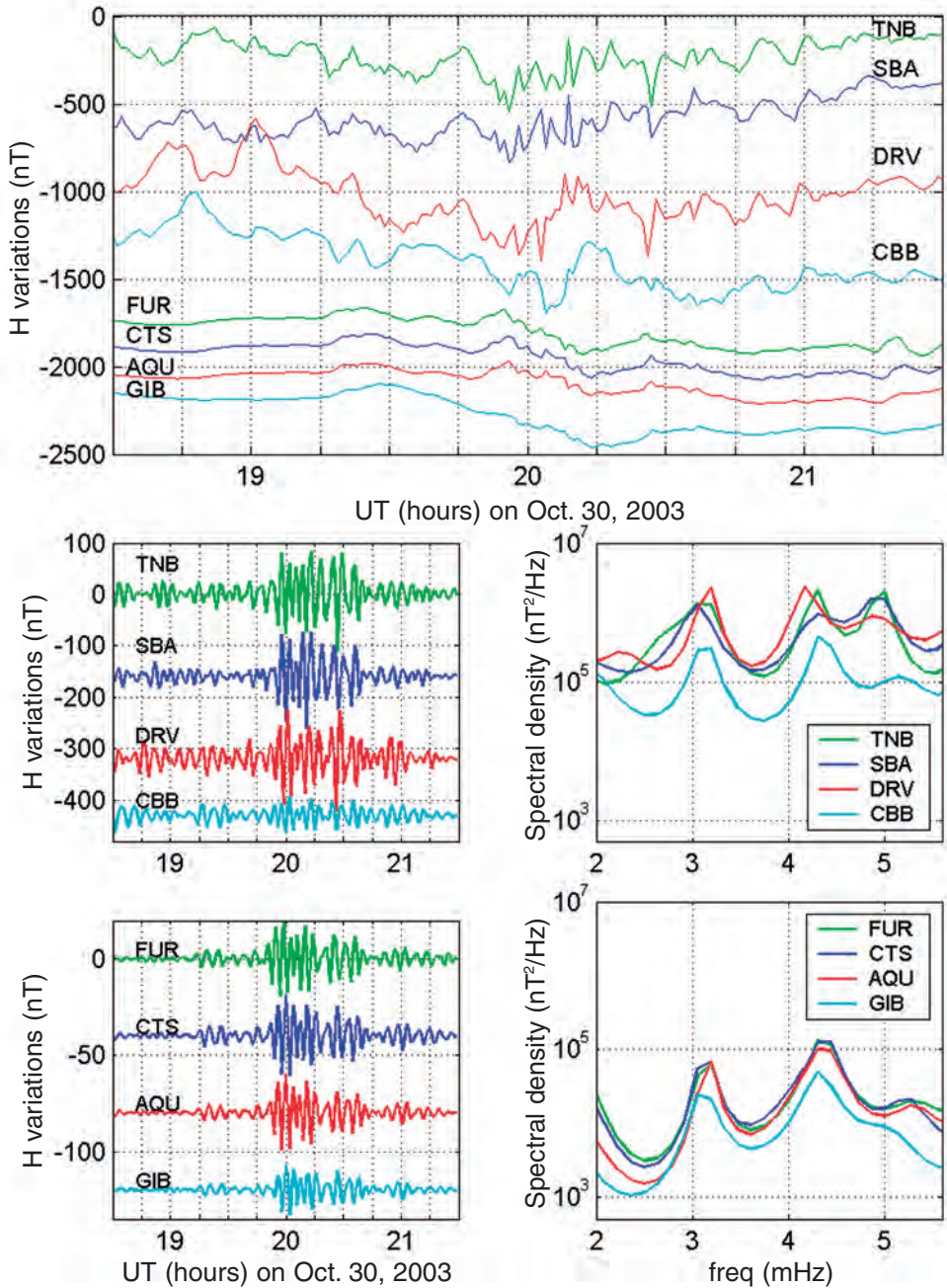
Fig. 8. Variations of the H component (unfiltered data, upper plot; 2-5 mHz filtered data, lower left plots) at four high latitude and four low latitude stations (table I) and corresponding power spectra from differenced data (plots on the right).
