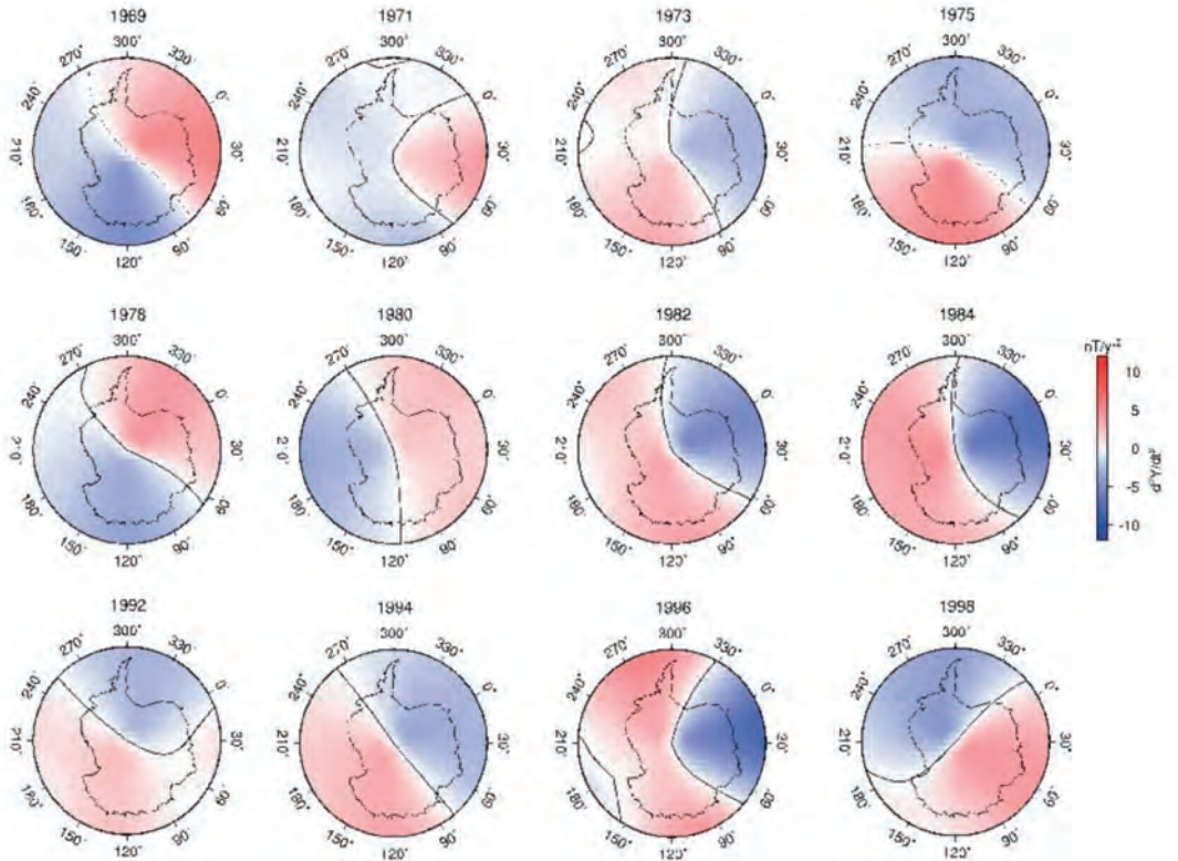
Fig. 2. Secular acceleration maps relative to the Y component over the Antarctic continent obtained using synthetic data given by the CM4 model. The solid line corresponds to the zero separating the zone characterized by negative (blue) and positive (red) values of secular acceleration.
