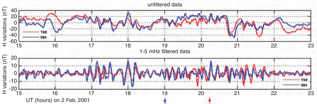
Fig. 7. Variation of the H component (unfiltered data, upper plot; 1-5 mHz filtered data, lower plot) at TNB (red line) and SBA (blue line). The red and blue arrows indicate the local geomagnetic noon at the two stations, respectively.
