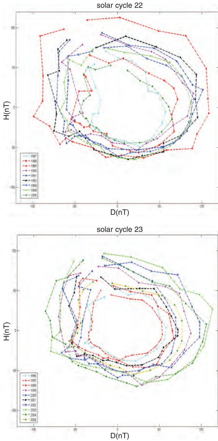
Fig. 6. Magnetic field hodograms for solar cycle 22 and solar cycle 23.
