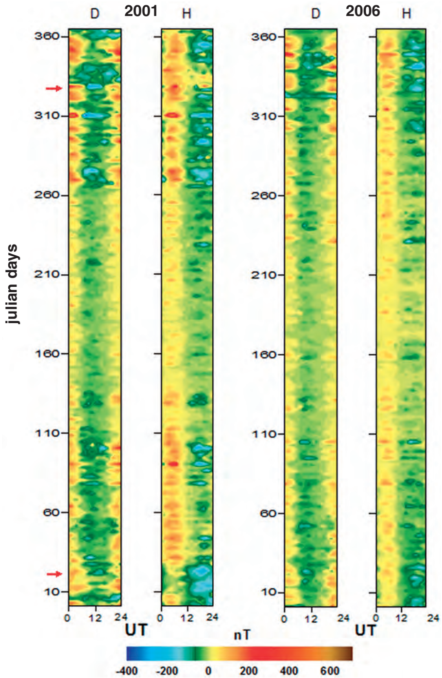
Fig. 5. Dynamic maps of diurnal variation for D and H components for 2001 and 2006 years.
