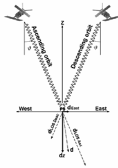
Fig. 7 Geometry of the acquisition system
