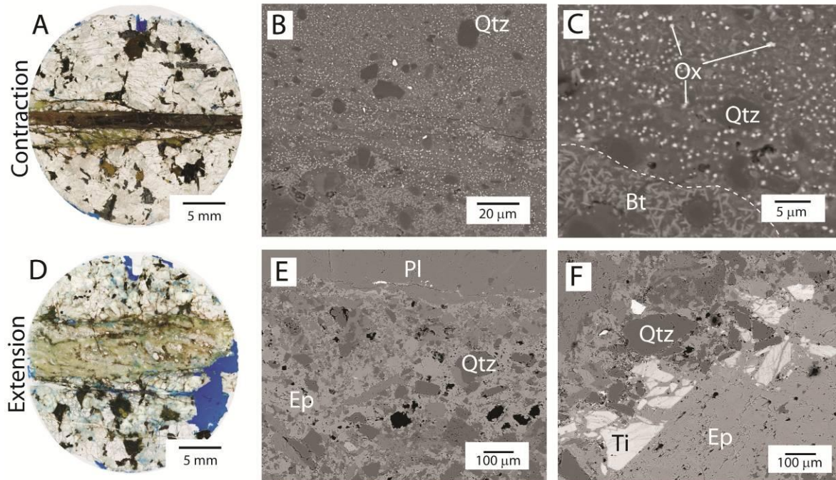
924 925 Figure 4: Sierran wavy fault microstructures from contractional (07_118d) and extensional 926 (07_118c) bends (see Fig. 1A for sample location). (A) Digital scan of thin section 07-118d, 927 showing dark PT vein and some associated green cataclasite along its boundaries. (B) - 928 Backscatter image of heterogeneous PT from sample 07-118d in a contractional bend, showing 929 two textural zones, and dark clasts of quartz (Qtz). (C) Close-up view of the boundary between 930 the compositional zones in B. Microlitic domain with biotite (Bt) microlites is below the dashed 931 line, and spherulitic domain with Fe-rich oxides (Ox) is above. (D) Digital scan of thin section 932 07-118c, showing pre-existing quartz mylonite overprinted by green cataclasite. No PT occurs 933 in this sample. (E) Cataclastic fabric consisting primarily of subangular quartz and feldspar 934 grains juxtaposed against a single plagioclase (Pl) grain (top) in the wall rock. Cataclasite is 935 extensively overgrown by epidote (Ep). (F) Epidote matrix in cataclasite with quartz and titanite 936 clasts. The titanite (Ti) is extensively fractured and the fractures are filled by epidote veins. 937
