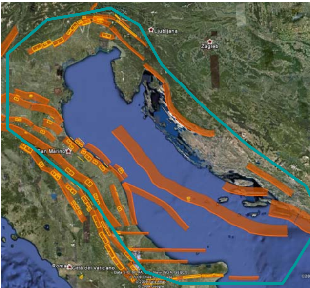
Fig. 2 Overview of the seismogenic sources of the Adria microplate included in DISS 3.1.0. The Individual Seismogenic Sources are represented with yellow rectangles, Composite Seismogenic Sources with red ribbons. The cyan polygon highlights the studied area.
