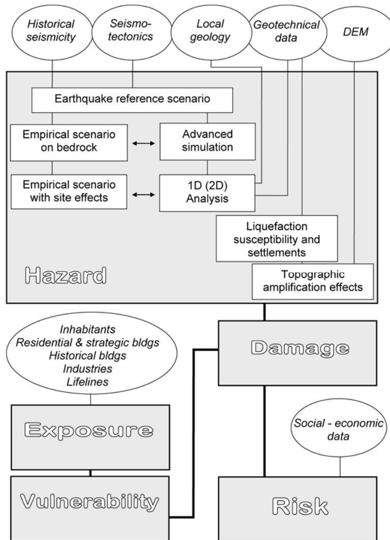
Figure 1 – Scheme of the seismic risk assessment method, illustrating the implementation of the WebGis applications for the Lake of Garda and western Liguria cases.
