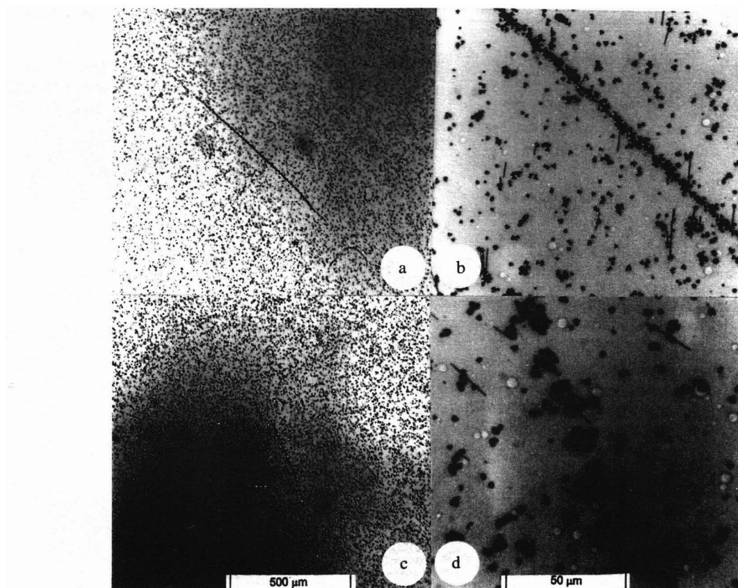
Fig. 12. (a) and (b) Alpha-particle traces that emanated from a natural thorium source.
