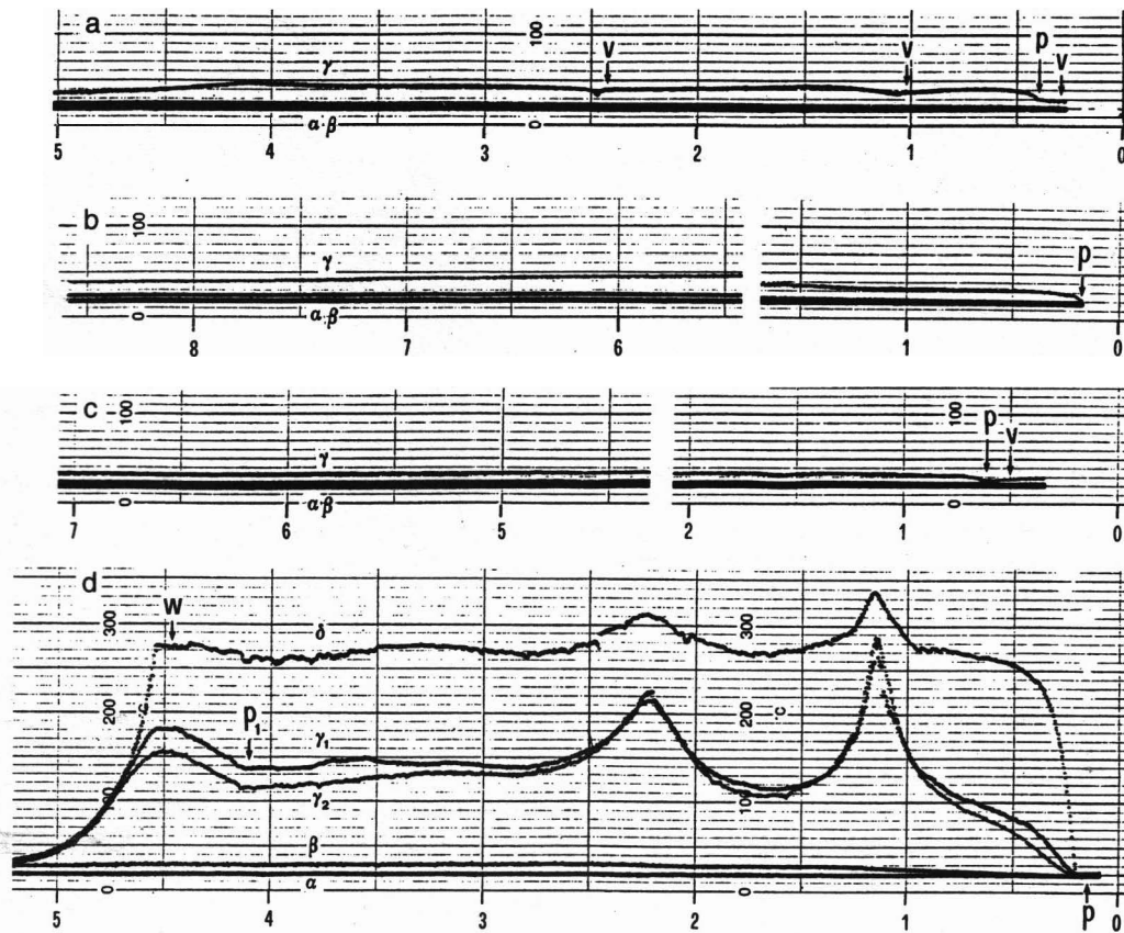
Fig. 7. Palladium coil. Temperature behavior. Abscissa: time in hours. Ordinate: temperature in degree Celsius. Curve \alpha : m temperature. Curve \beta : barycenter of the brass disk (2.6 kg). Curve \gamma : intermediate turn of the coil (0.203 kg). In (d), p_1 indicates the increase imposed on the hydrogen pressure inside the coil, from 10.4 to 12.5 bars. Curve \delta : electric heater at 1 cm from contact with the coil. Curve \gamma_1 : point of the coil at 1 cm from contact. Curve \gamma_2 : point of the coil diametrically opposite to the former contact point. In w, the electric heater has been switched off. Symbols: p: pressure; v: vacuum; w: heating. Other data in Table III.
