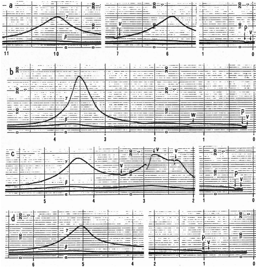
Fig. 6. Palladium coil. Temperature behavior. Abscissa: time in hours. Ordinate: temperature in degrees Celsius. Curve a: room temperature. Curve beta: barycenter of the brass disk (2.6 kg). Curve gamma: intermediate turn of the coil (0.203 kg). Symbols: p: pressure; v: vacuum; w: heating. Other data in Table III.
