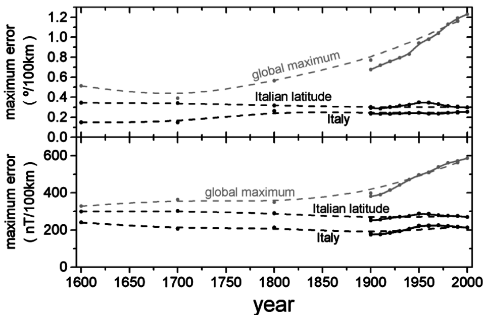
Fig. 4. Evolution of the maximum values of (a) angular and (b) intensity relocation errors through time according to the GUFM1 and IGRF-9 models (dashed and continuous lines respectively). Bold (Italian maxima), dark grey (Italian latitude maxima), light grey (global maxima).
