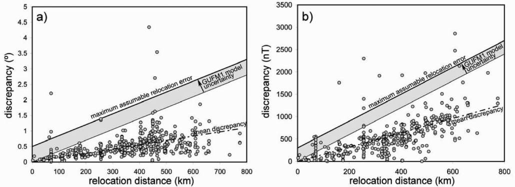
Fig. 5. Angular (a) and intensity (b) discrepancy between relocated data from the Italian catalogue and GUFM1 values at Viterbo as a function of relocation distance. Shifted line of maximum assumable relocation error has been plotted to identify anomalous data.
