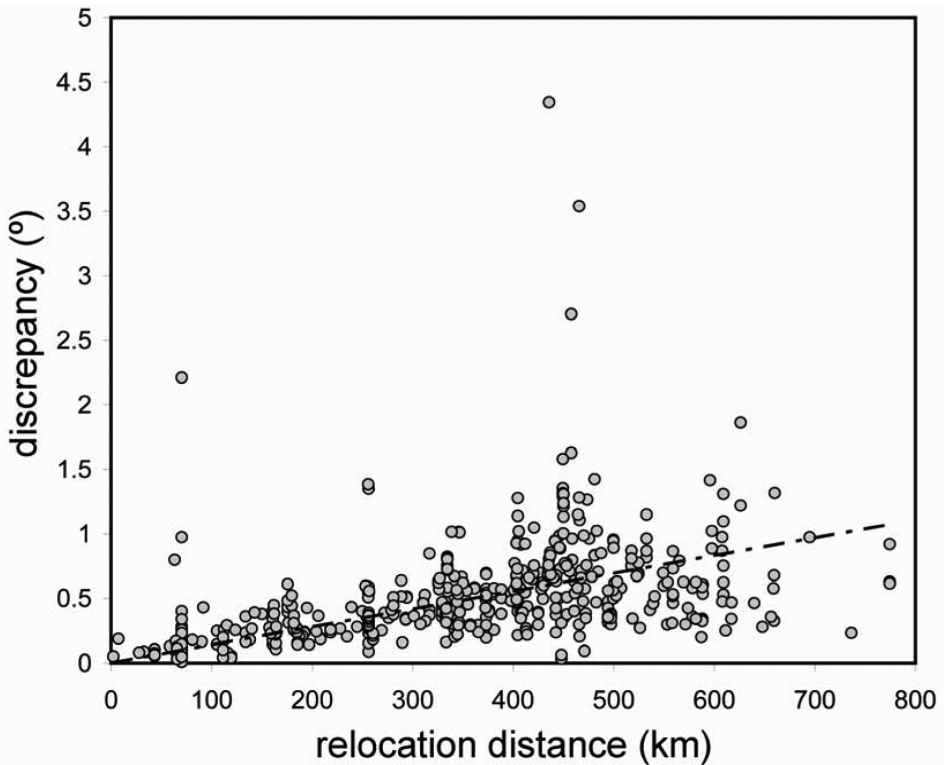
Fig. 3. Angular discrepancy between the relocated Italian-catalogue data and GUFM1 values at Viterbo as a function of relocation distance. Correlation is apparent.
