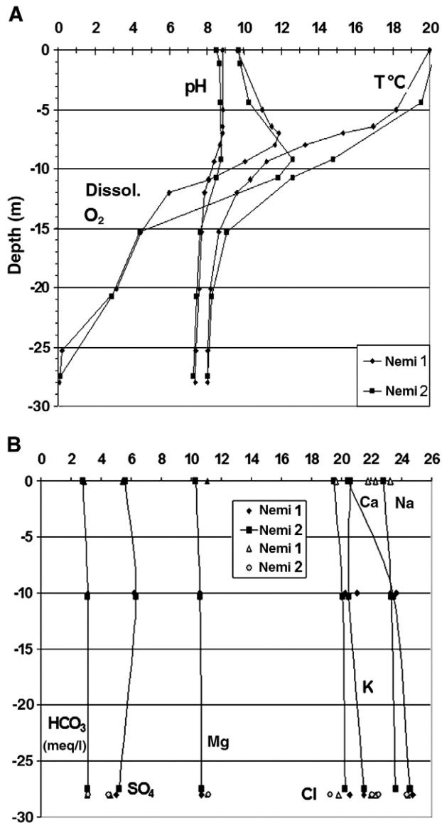
Fig. 9. A: Variation with depth of T, pH and dissolved O_2 measured in May 2004 in the Lake of Nemi. B: Variation with depth of the concentration of the anions and cations in mg/l (except for HCO_3 in meq/l) in the Lake Nemi waters. See Fig. 10 for the location of water sampling points.
