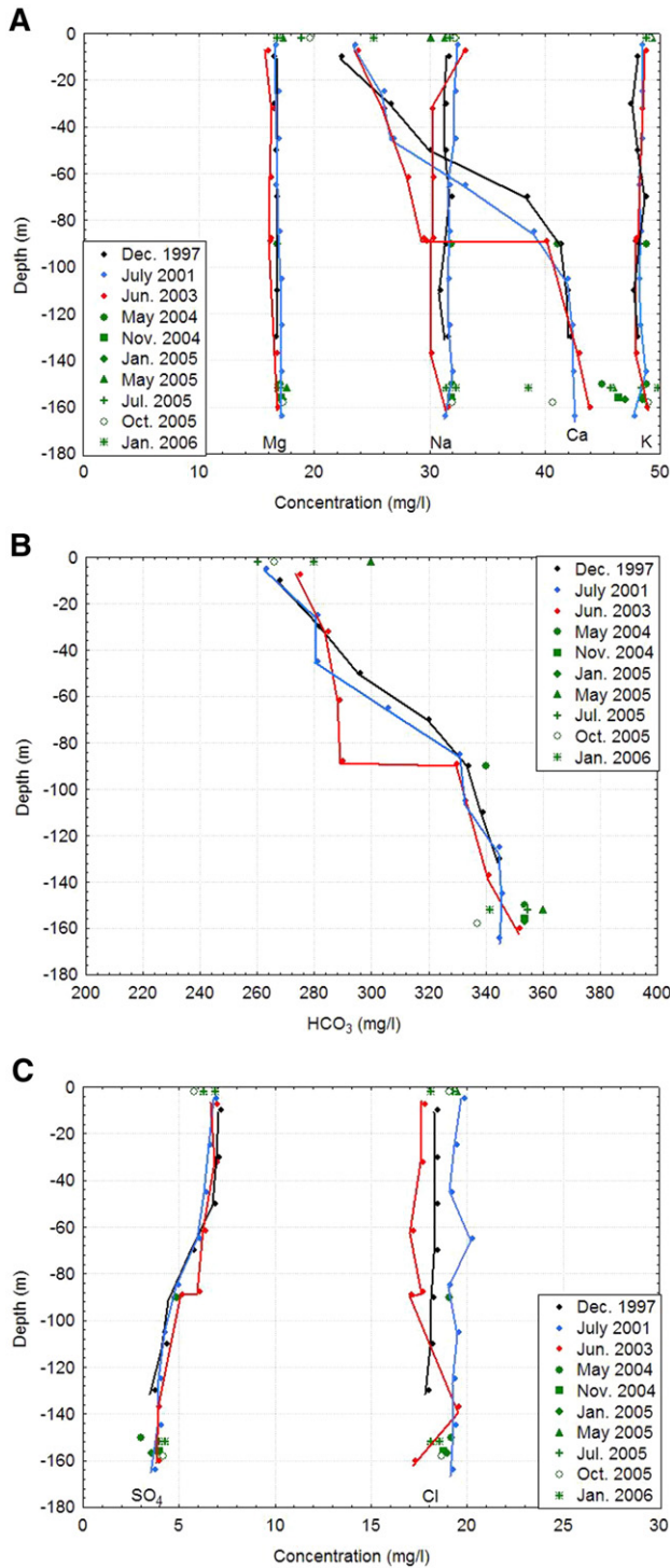
Fig. 4. Variation with depth of the concentration of cations (A), \text{HCO}_3 (B) and anions (C) in the Lake Albano waters from July 2001 to January 2006. The 1997 profiles are from Cioni et al. (2003).
