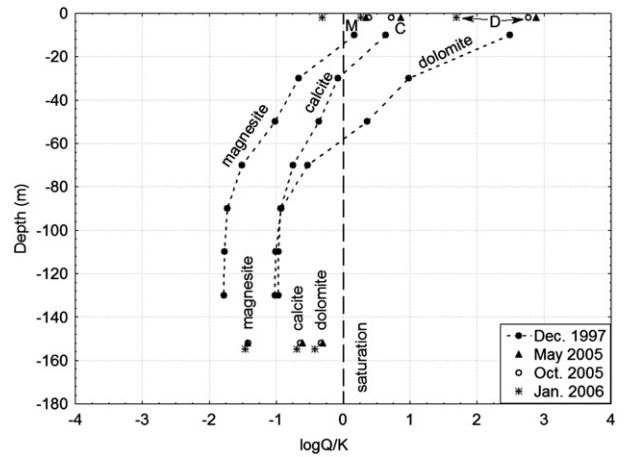
Fig. 5. Saturation index of carbonate minerals in Lake Albano water calculated following the procedures of Cioni et al. (2003).
