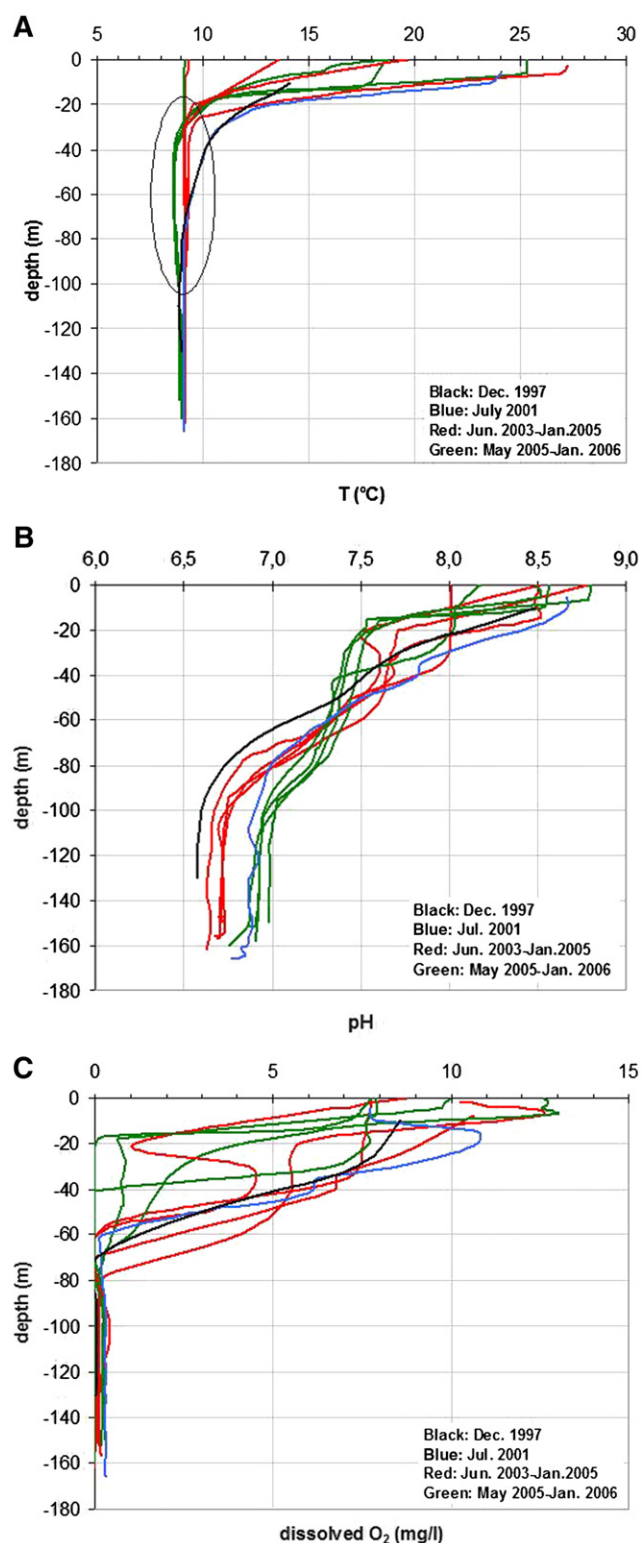
Fig. 3. Vertical profiles measured in the deepest part of Lake Albano (48 and A03 in Fig. 2) in 2001–2006. A: Variation with depth of temperature; B: variation with depth of pH; C: variation with depth of the dissolved O 2 . The 1997 profiles are from Cioni et al. (2003).
