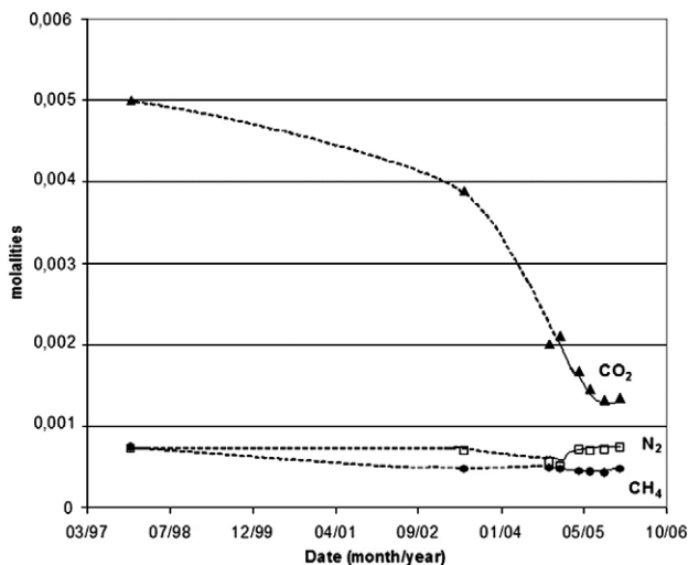
Fig. 7. Concentration (molalities) of dissolved CO 2 , N 2 and CH 4 in the deepest water sample collected in the 1997–January 2006 surveys (depth range = 152–160 m). The 1997 data are from Cioni et al. (2003).
