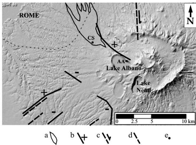
Fig. 1. Digital elevation model of the Alban Hills volcanic district with the location of the crater lakes Albano and Nemi. a) Ciampino plain Holocene syn- and inter-eruptive lahar deposits; b) structural highs (+) and lows (-) of the carbonate basement revealed by gravity anomalies; c) main strike-slip faults; d) main normal faults; e) gas manifestation sites (CS=Cava dei Selci, AA=Acqua Acetosa).
