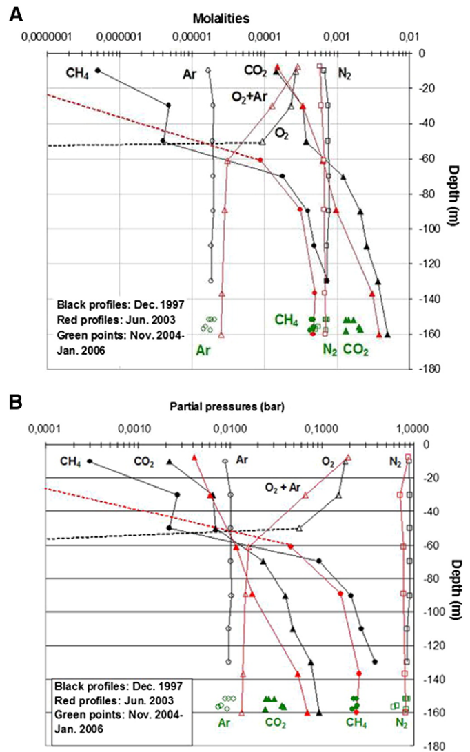
Fig. 6. Variation with depth of the content (molalities A) and partial pressure (B) of dissolved gases ( \text{CO}_2 , \text{N}_2 , \text{CH}_4 , \text{O}_2 and Ar) in the Lake Albano waters. In the June 2003 profile the sum of \text{O}_2 and Ar is reported but direct measurements of dissolved \text{O}_2 (Fig. 3C) indicate that the \text{O}_2 content is zero below 70 m depth.
