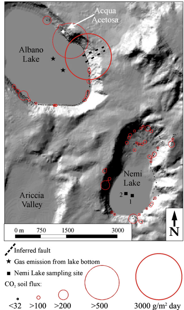
Fig. 10. Diffuse CO_2 soil degassing from the shores of the crater lakes Albano and Nemi. The diameter of the circles expresses the CO_2 soil flux values (see scale). Black dots: measurement points and flux lower than 32 \text{ g}\cdot\text{m}^{-2} \cdot \text{day}^{-1} (background); black square: sampling sites of Nemi waters.
