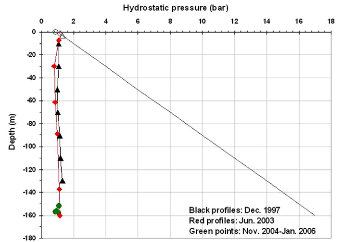
Fig. 12. Variation with depth of the total pressure of the gases dissolved in the Lake Albano water in the period December 1997–January 2006, compared to the hydrostatic pressure. Open symbols on the upper part of the hydrostatic pressure line indicate the depth at which gas would have exsolved should the deepest water have been brought to the surface. The 1997 profile is from Cioni et al. (2003).
