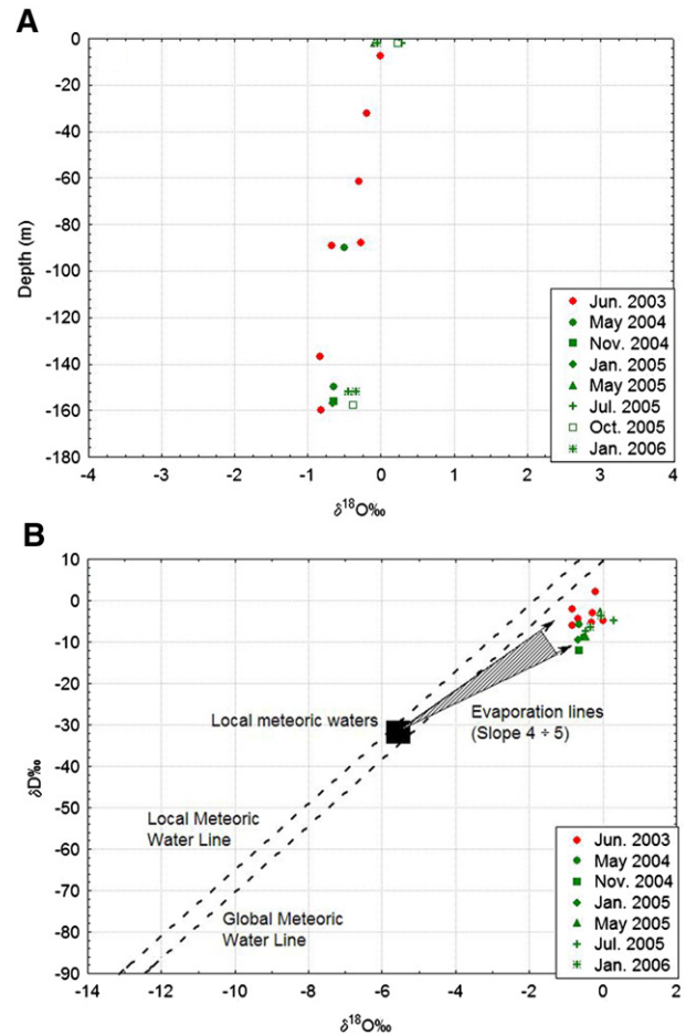
Fig. 8. A: Variation with depth of the oxygen isotopic composition in the water samples of Lake Albano collected in June 2003–January 2006 surveys (analytical error: ±0.1). B: Isotopic composition of oxygen vs deuterium in the waters of Lake Albano and Nemi. The isotopic changes induced by evaporation are indicated. The isotopic composition of the local meteoric waters is from Longinelli and Selmo (2003).
