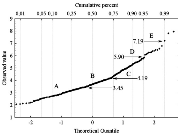
Fig. 11. Normal probability plot (log scale) of the soil flux measurements (376 sampling points) on the shores of Albano and Nemi crater lakes; see Fig. 10 for point location.
