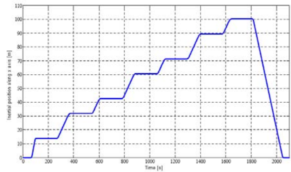
Figure 7. Helicopter position along inertial frame x axis.
