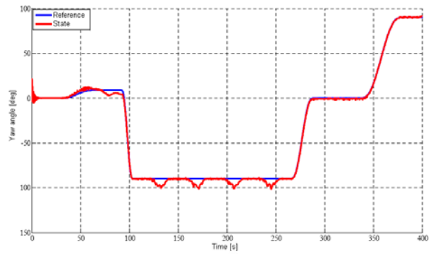
Figure 13. Roll angle tracked by the control system wrt. the reference trajectory.
