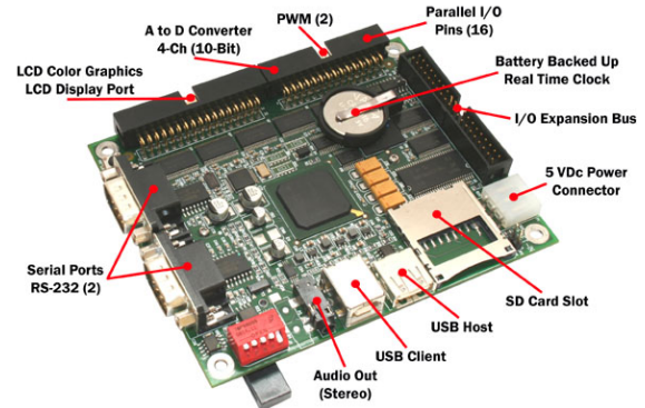
Figure 3. The RLC 520 MHz XScale-Mini processor.
