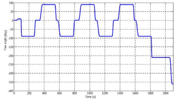
Figure 8. Helicopter yaw angle along the reference trajectory.
