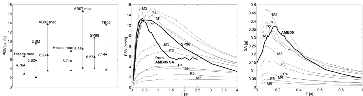
Figure 2 Comparison among PGV values (m, m ± s.d.) evaluated by DSM, Hisada method and empirical models AB07 (mean and maximum horizontal values), SP96 and TB02 (maximum values) (left); pseudo velocity spectra PSV obtained by DSM (thin lines), SP96 and AMB05 (from SA) (centre); acceleration spectra SA by DSM (thin lines) and AMB05 (bold line) (right)
