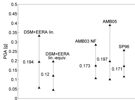
Figure 3 Comparison between PGA values (mean horizontal component) obtained by 1D linear and linear-equivalent analyses with empirical predictions
