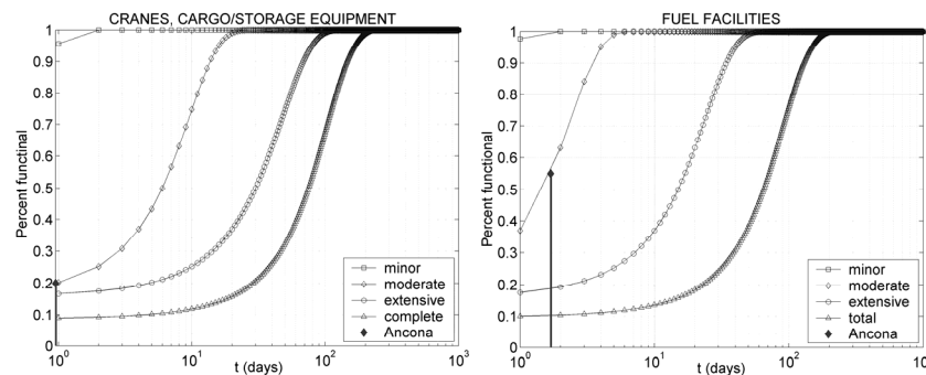
Figure 6 Restoration curves and expected time for serviceability restoration of the most damaged structures in the Ancona harbor: cargo/storage equipment (left), fuel facilities (right)
