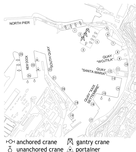
Figure 4 Location of the harbour components analysed in-damage assessment
