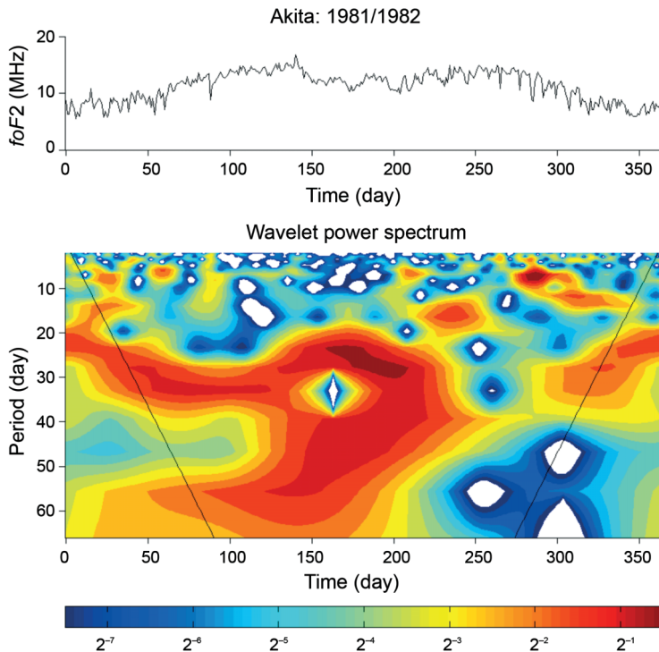
Fig. 1. Planetary wave type activity inferred from f_oF2 for Akita, 1 July 1981-30 June 1982, Morlet wavelet transform. Top panel: time series of raw f_oF2 data. Bottom panel: wavelet power spectrum of the planetary wave activity changing by colour from white and black-blue (minimum values) through green to red and black-red (maximum values). Wavelet power spectrum is normalized to 1.
